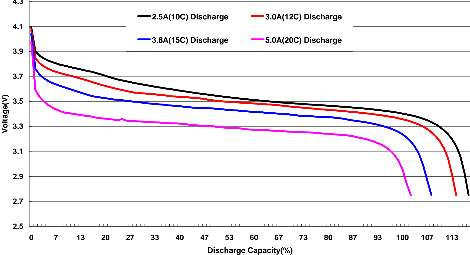
FB250XL 10C-20C Discharge Curves
