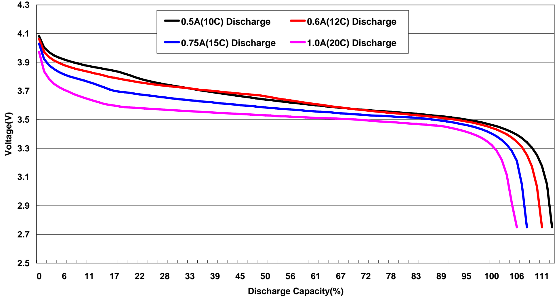
FB50XL 10C-20C Discharge Curves
