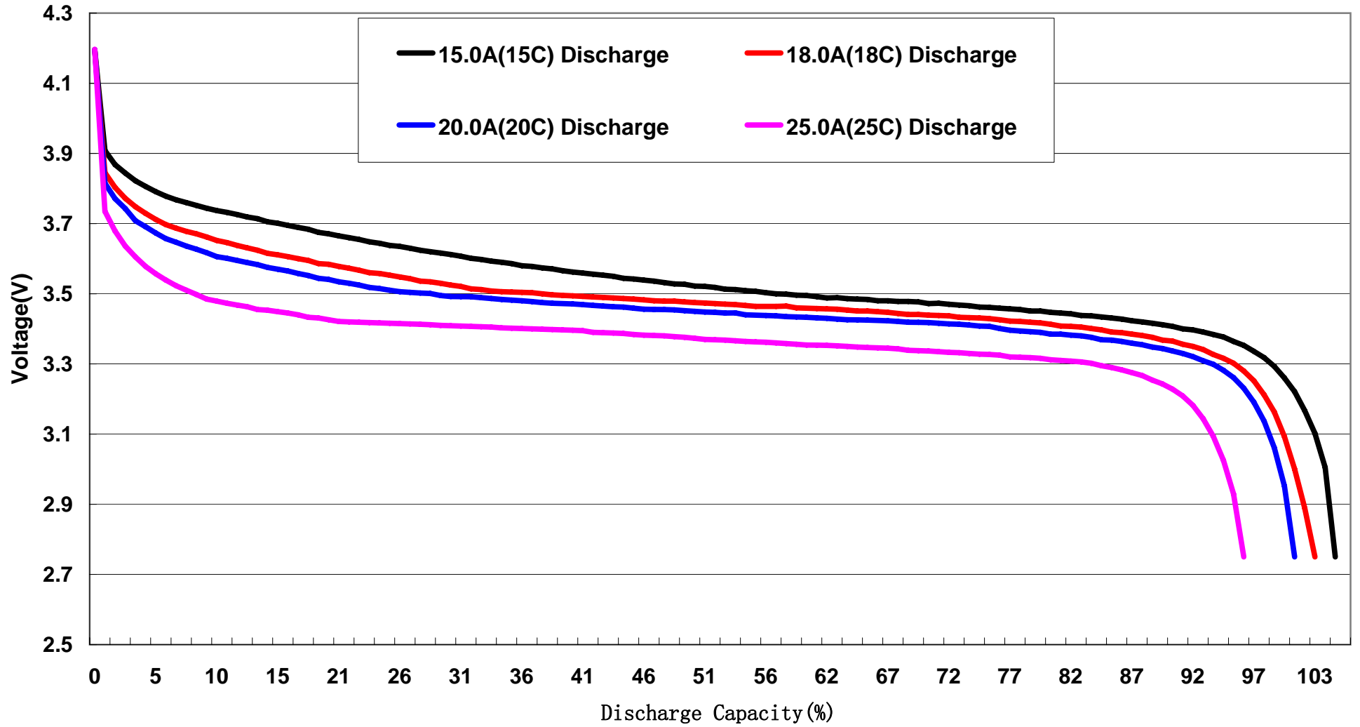
FB1000HP 15C-25C Discharge Curves
