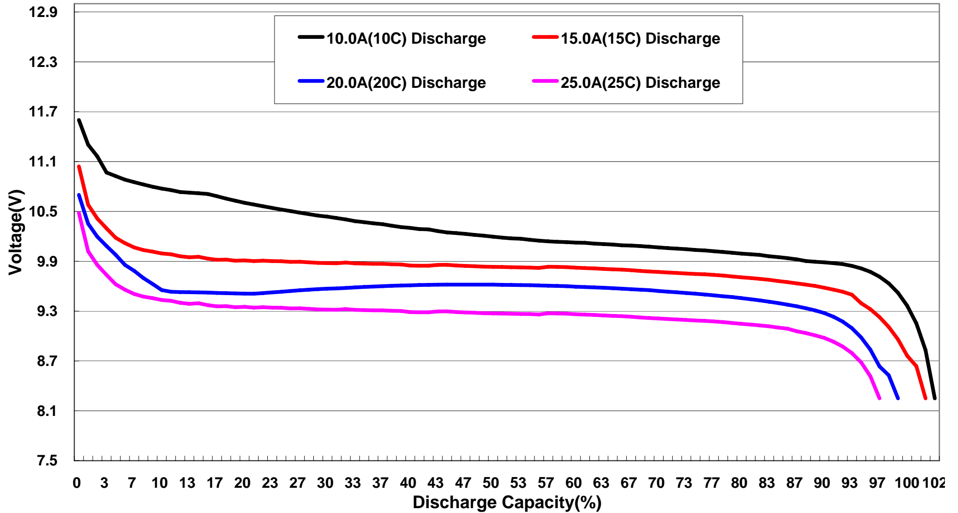
FB1000HP-3S 10C-25C Discharge Curves
