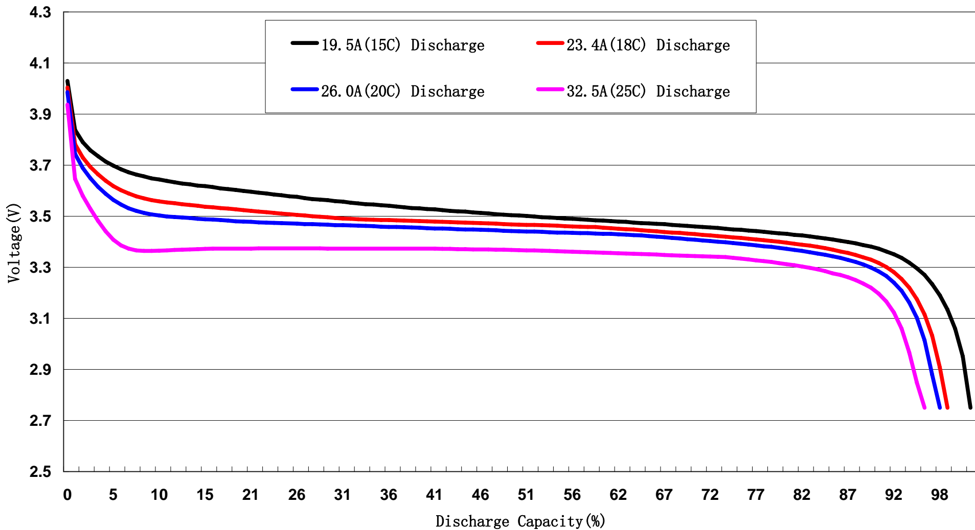
FB1300HP 15C-25C Discharge Curves
