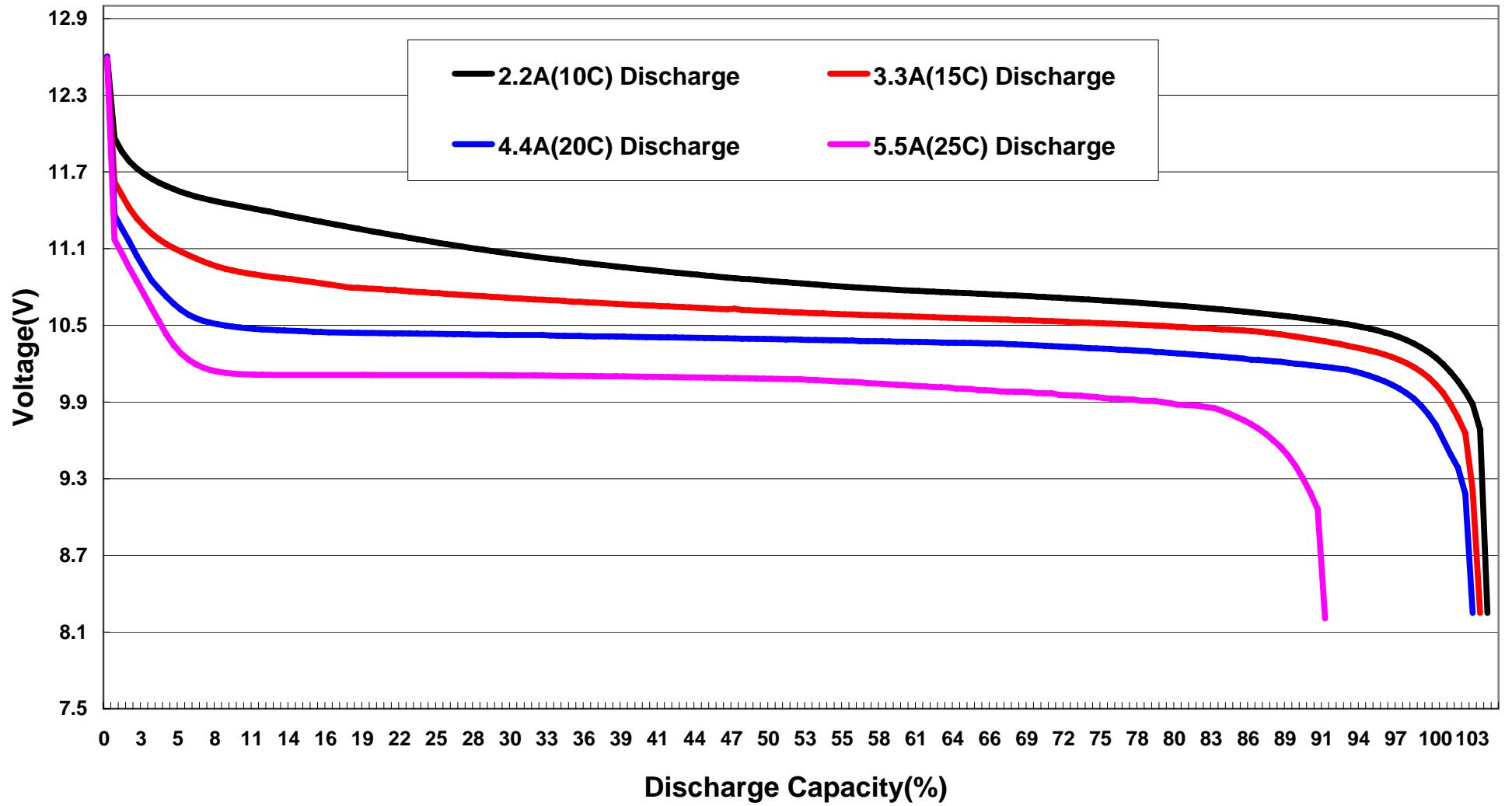
FB2200HP-3S 10C-25C Discharge Curves
