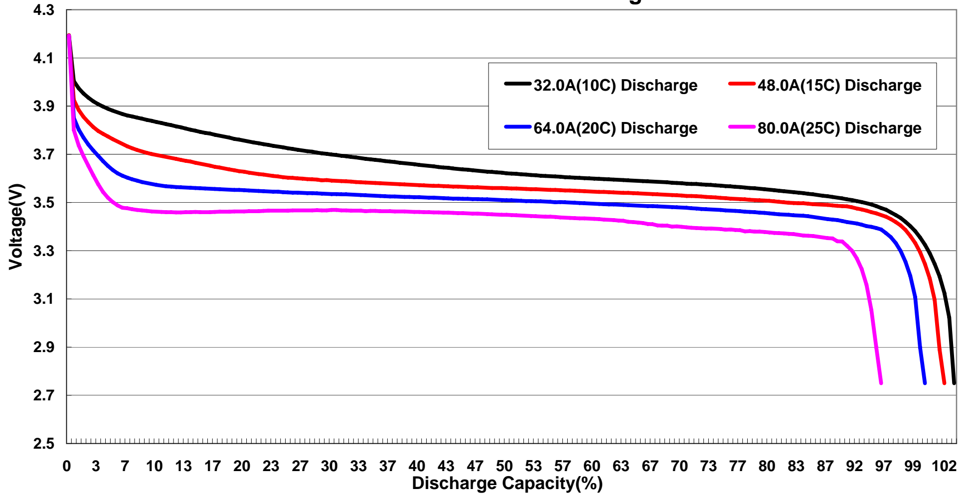
FB3200HP-1S 10C-25C Discharge Curves
