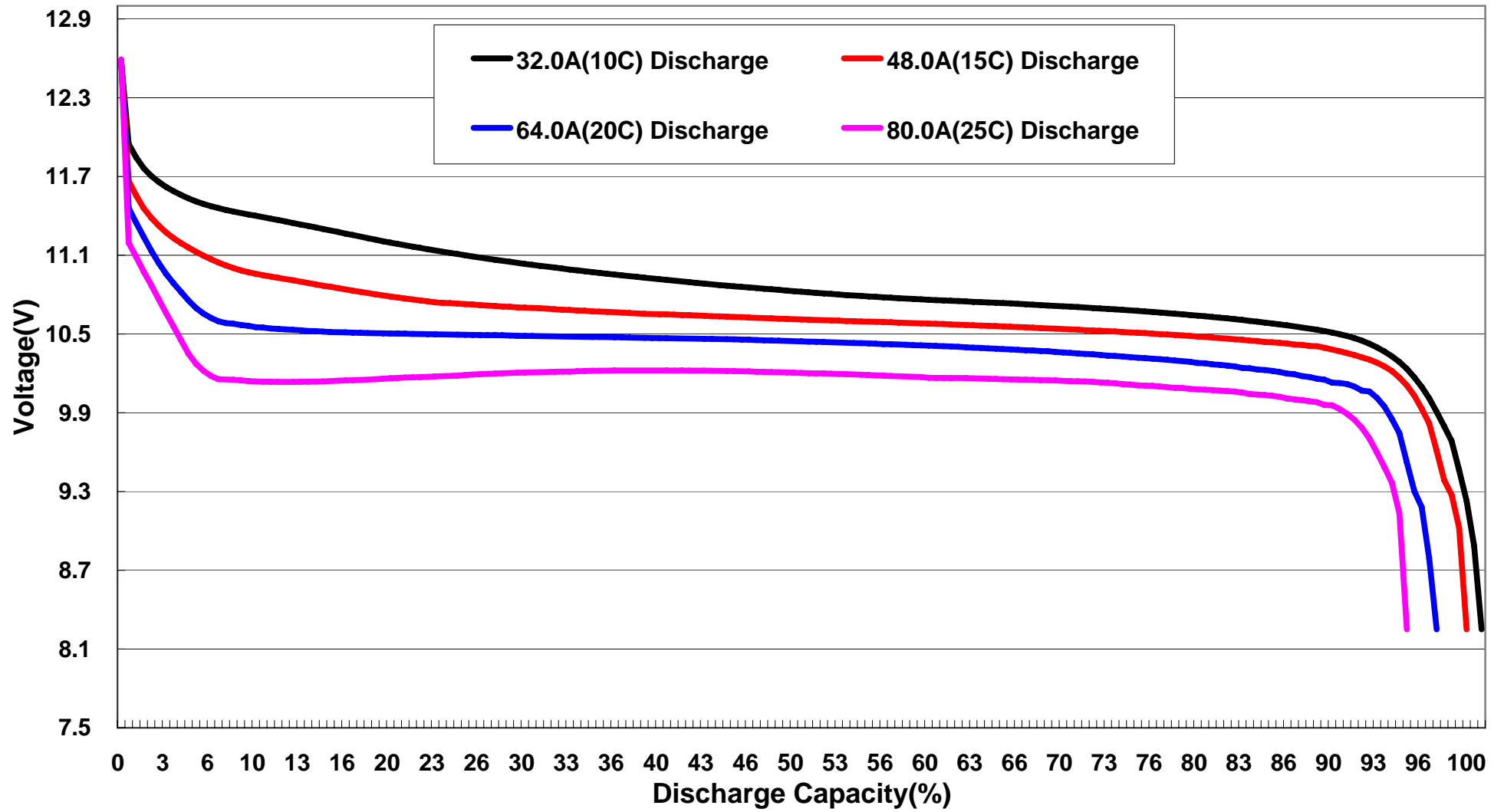
FB3200HP-3S 10C-25C Discharge Curves
