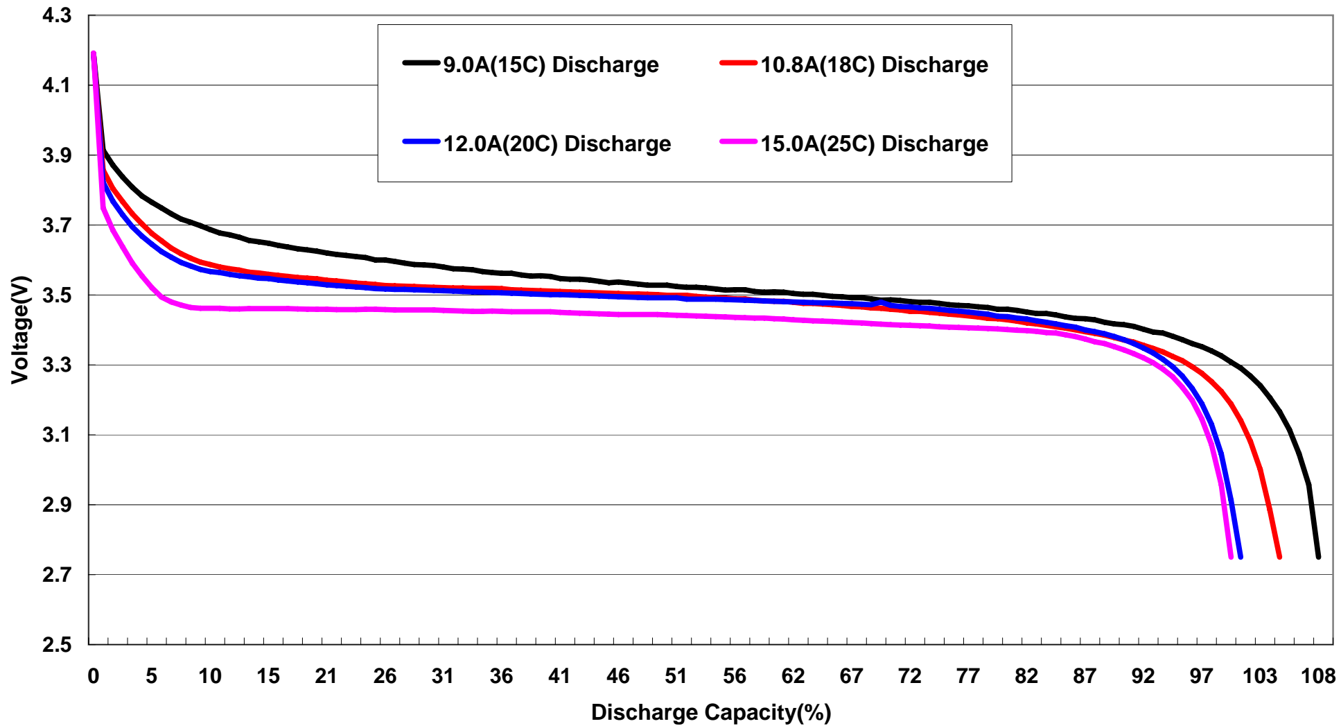
FB600HP 15C-25C Discharge Curves
