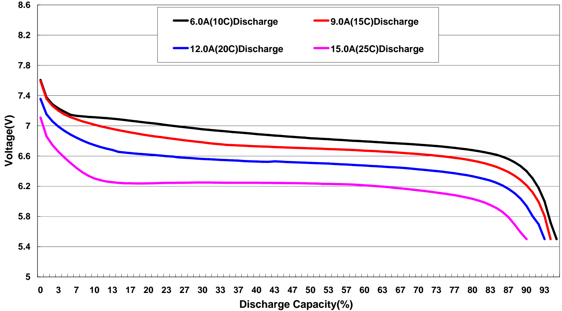
FB600HP-2S 10C-25C Discharge Curves
