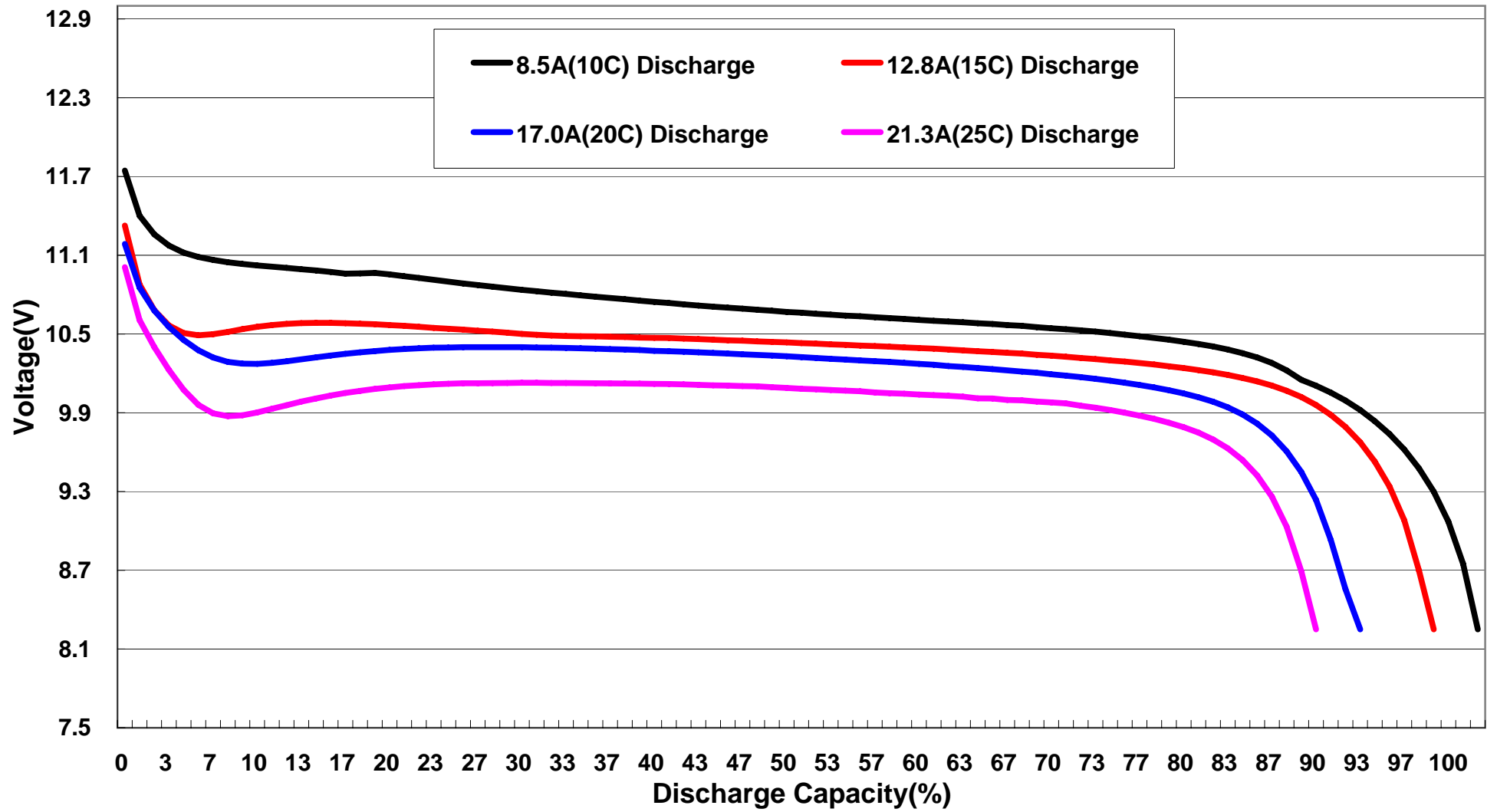
FB850HP-3S 10C-25C Discharge Curves
