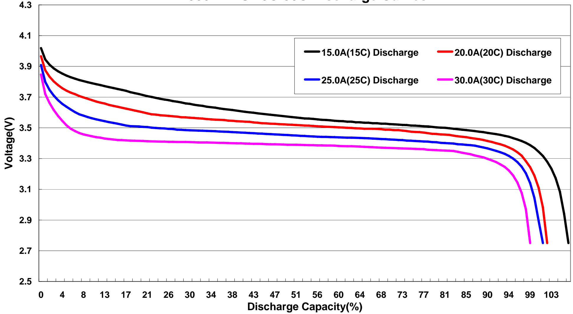
FB1000XP-1S 15C-30C Discharge Curves
