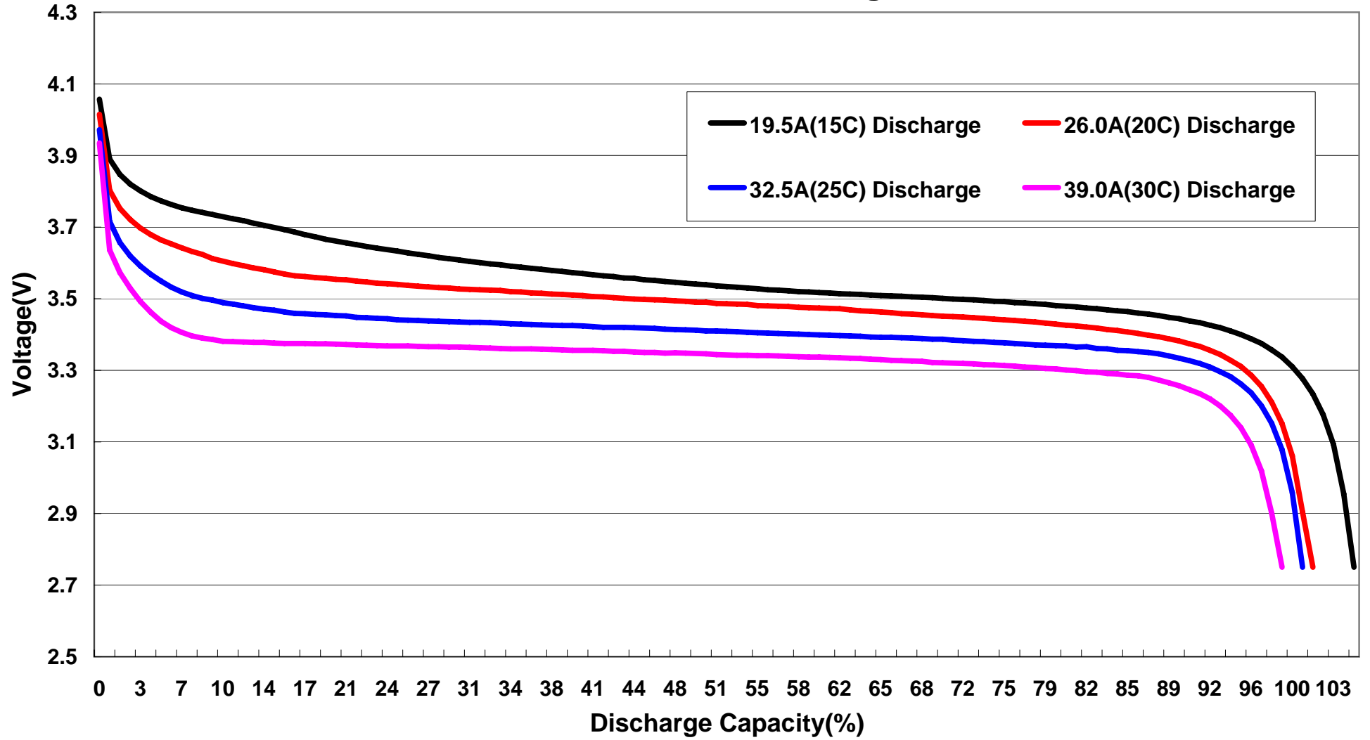
FB1300XP-1S 15C-30C Discharge Curves
