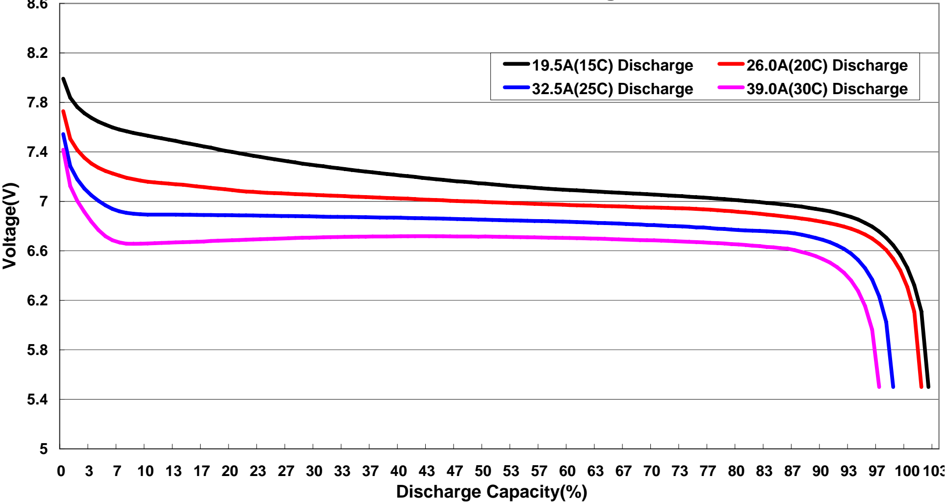
FB1300XP-2S 15C-30C Discharge Curves
