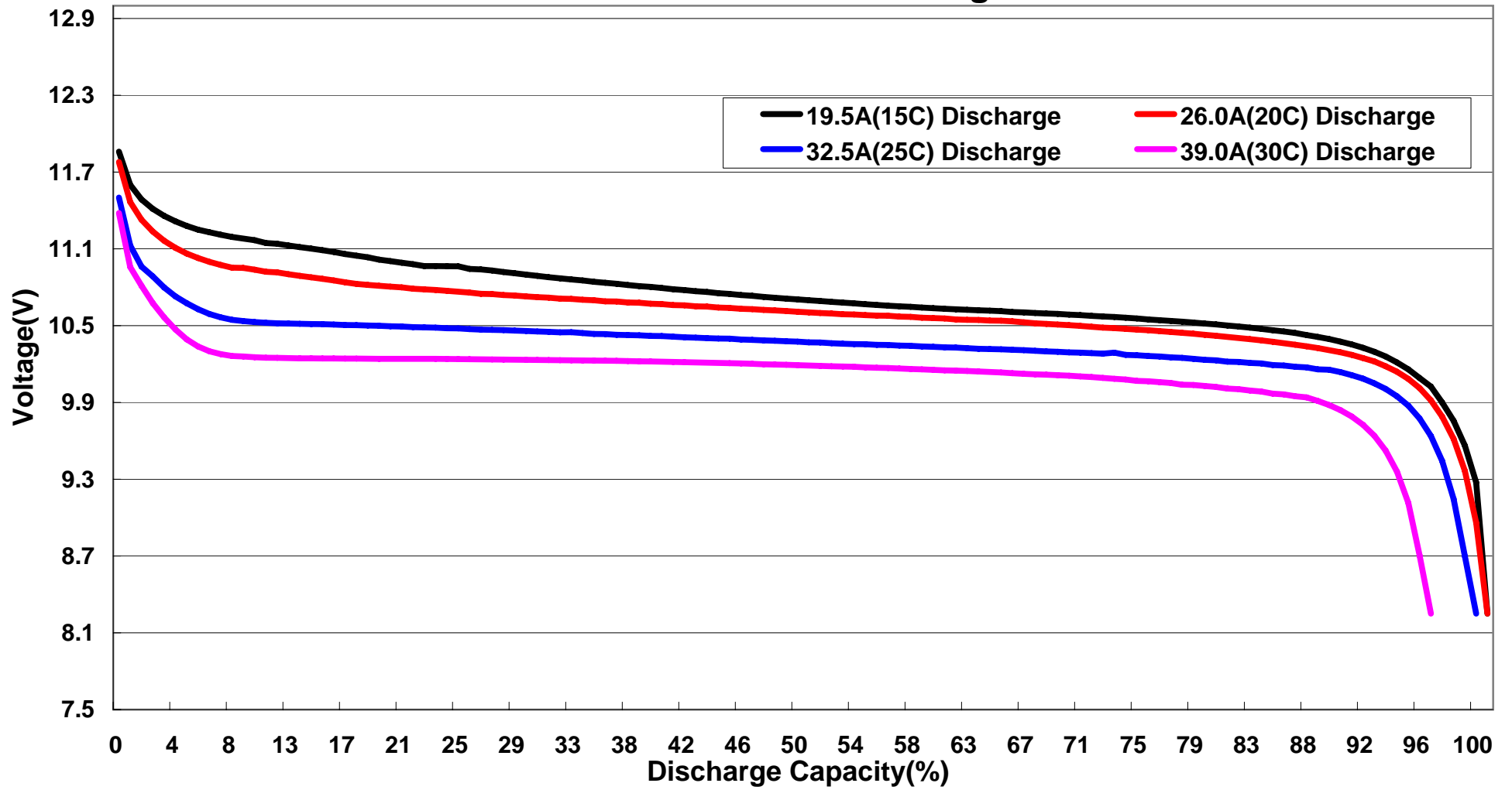
FB1300XP-3S 15C-30C Discharge Curves
