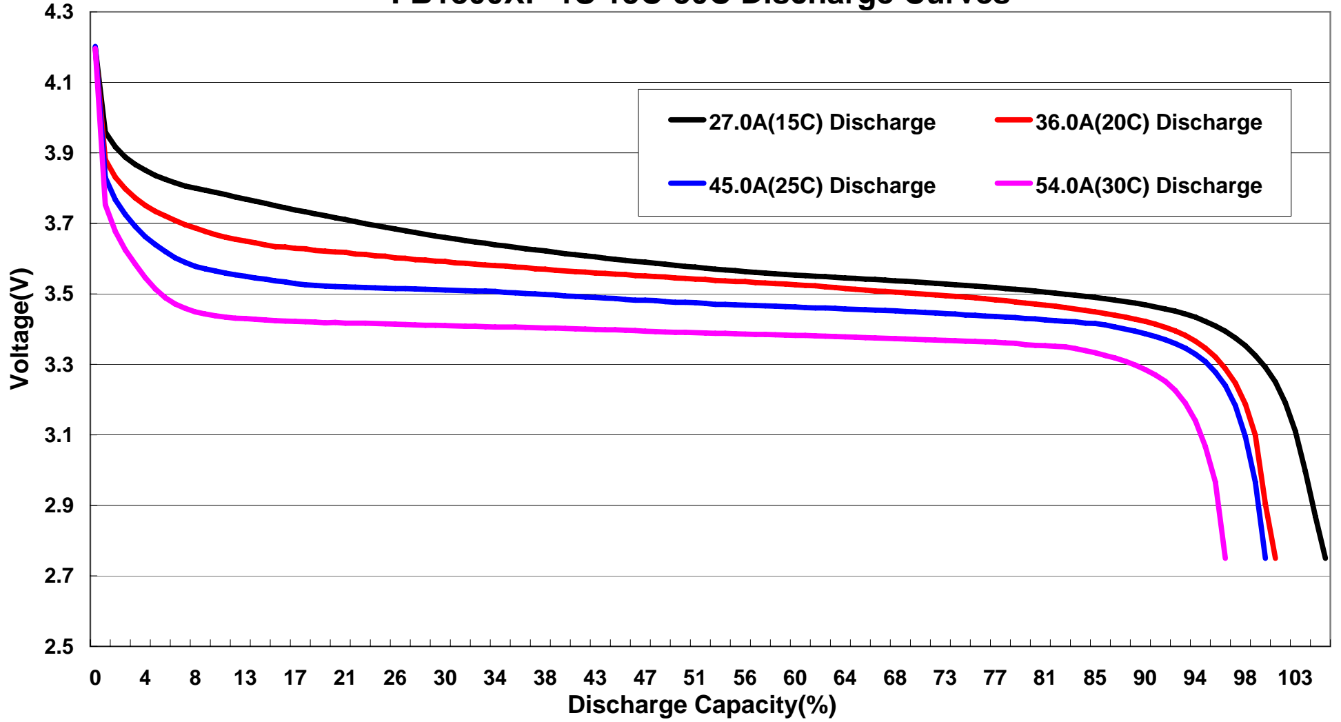
FB1800XP-1S 15C-30C Discharge Curves
