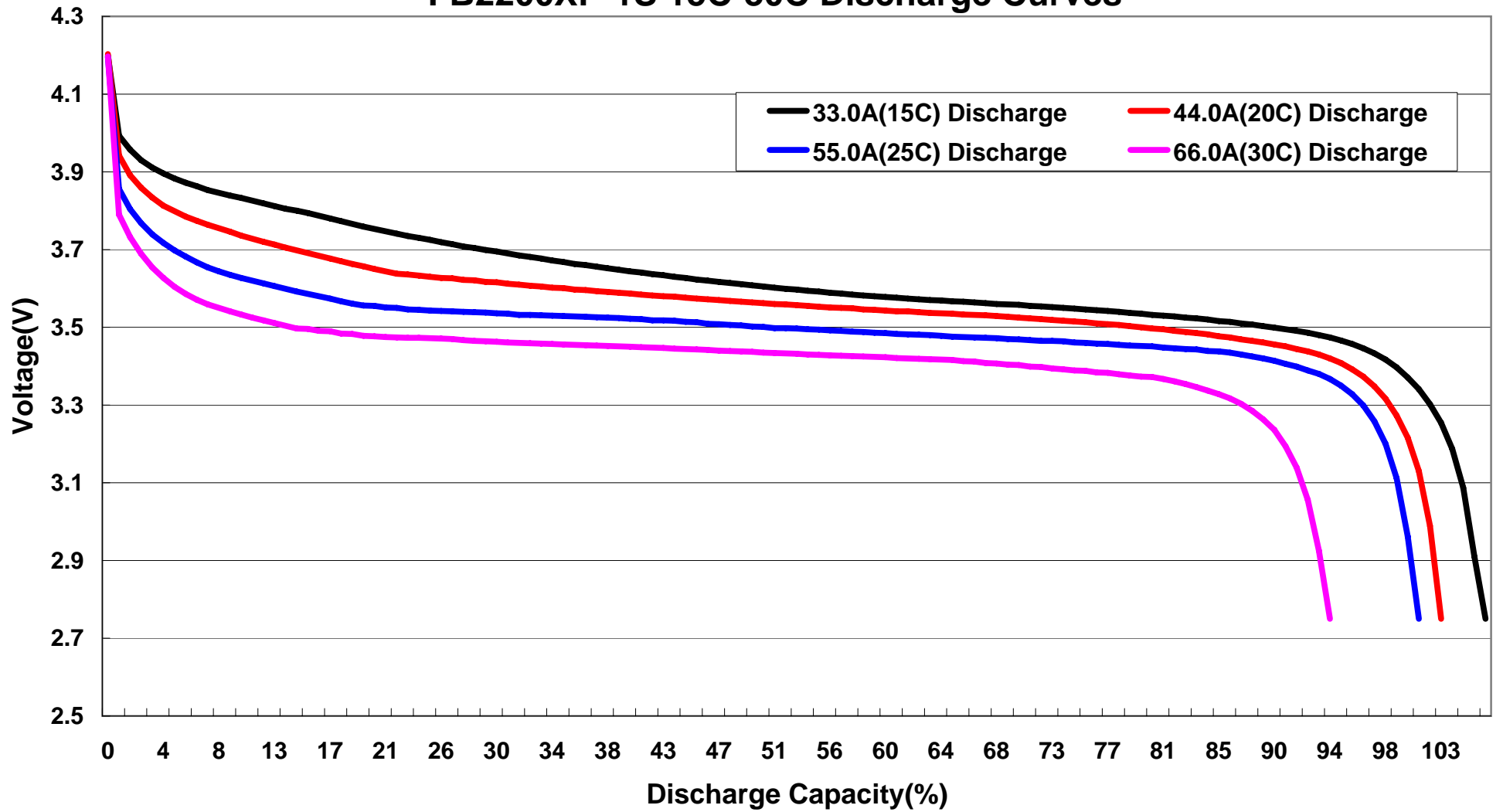
FB2200XP-1S 15C-30C Discharge Curves
