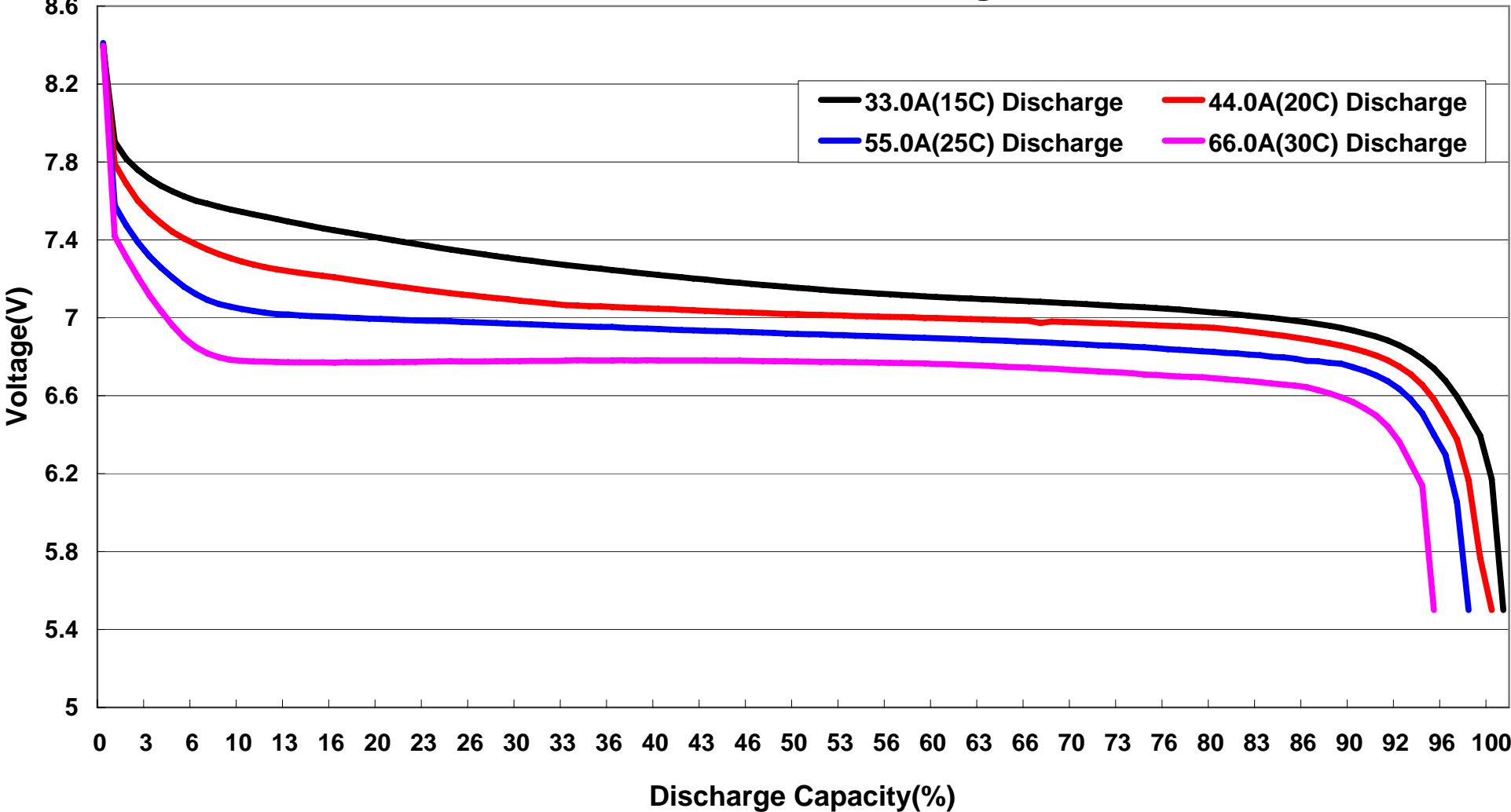
FB2200XP-2S 15C-30C Discharge Curves
