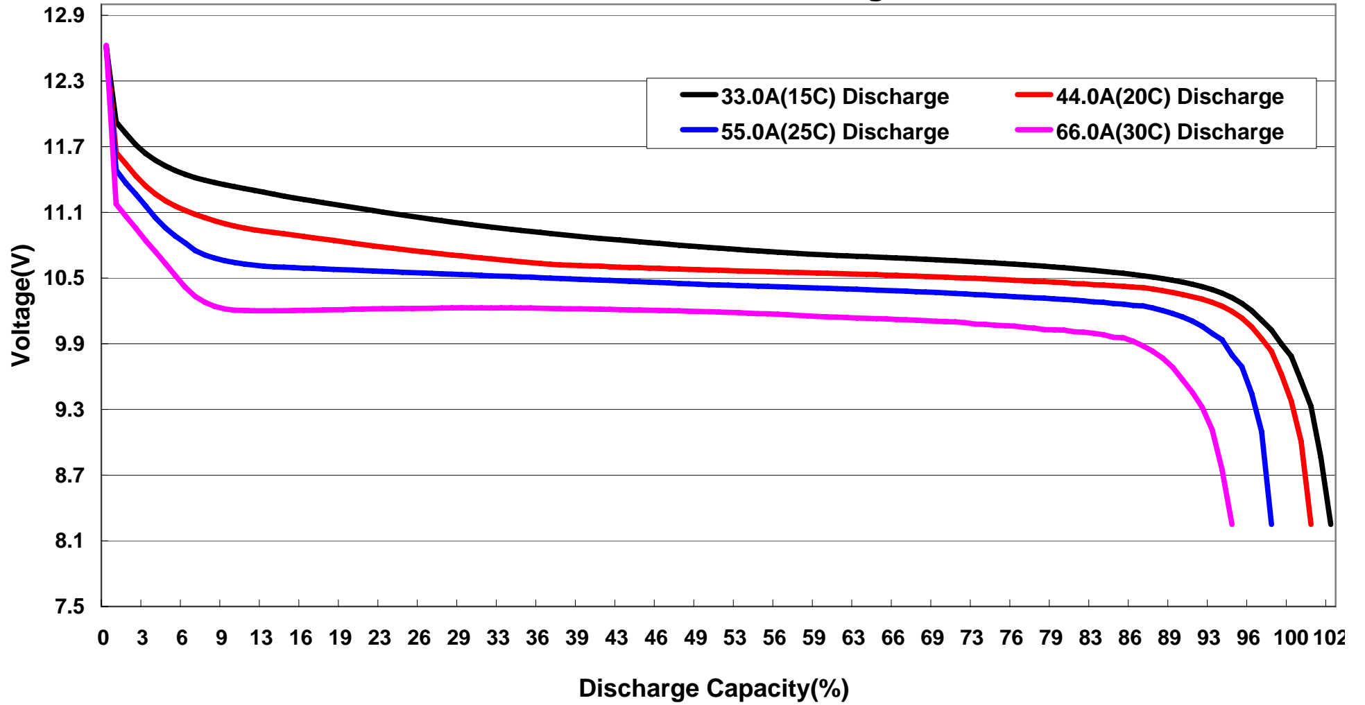
FB2200XP-3S 15C-30C Discharge Curves
