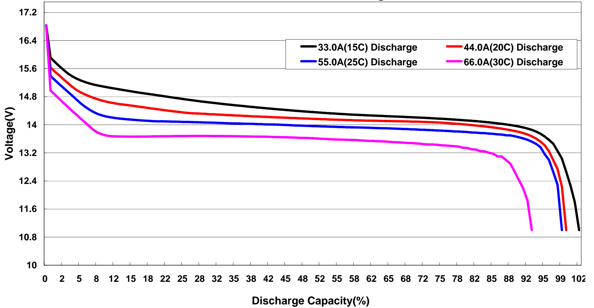
FB2200XP-4S 15C-30C Discharge Curves
