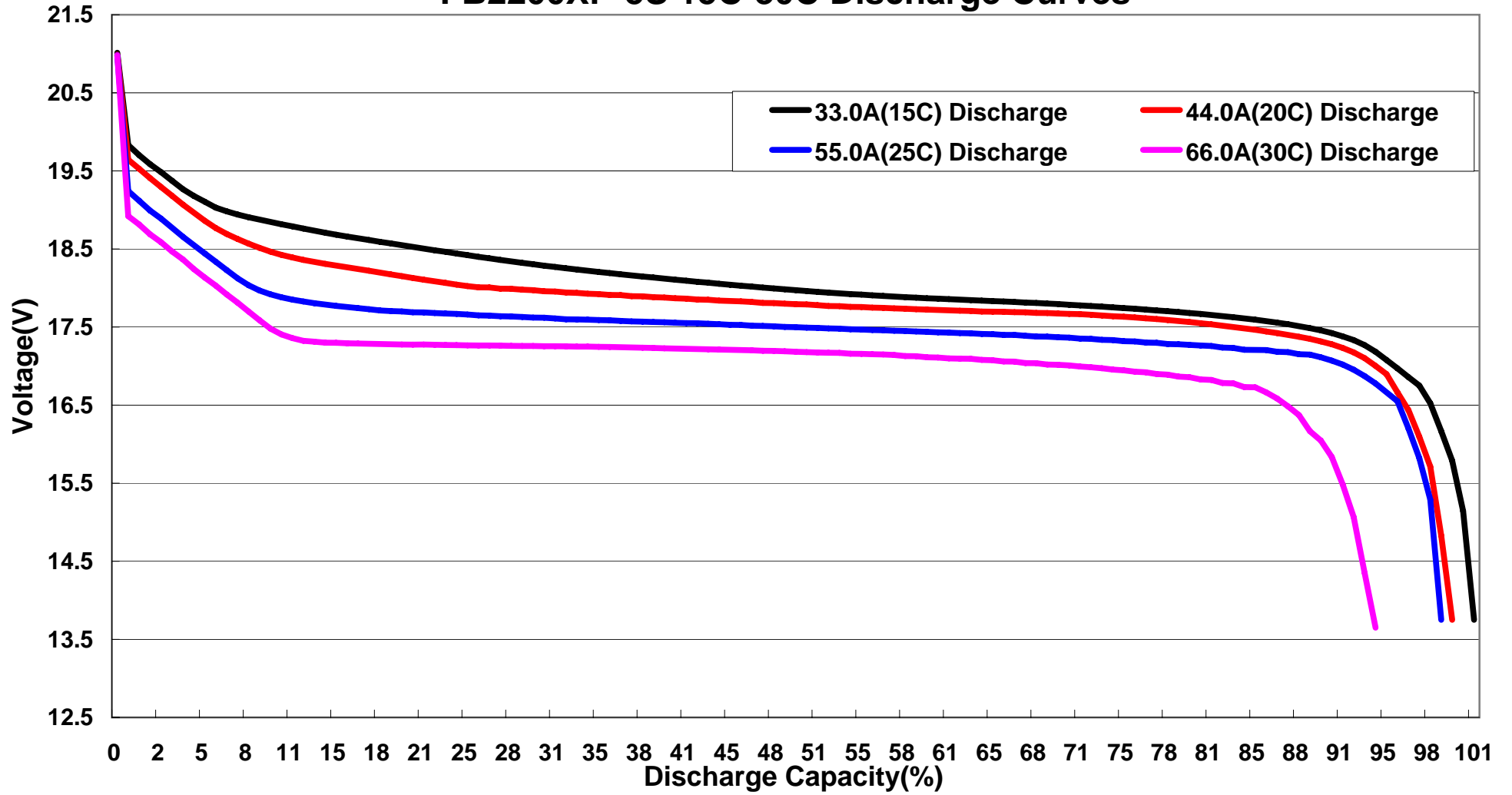
FB2200XP-5S 15C-30C Discharge Curves
