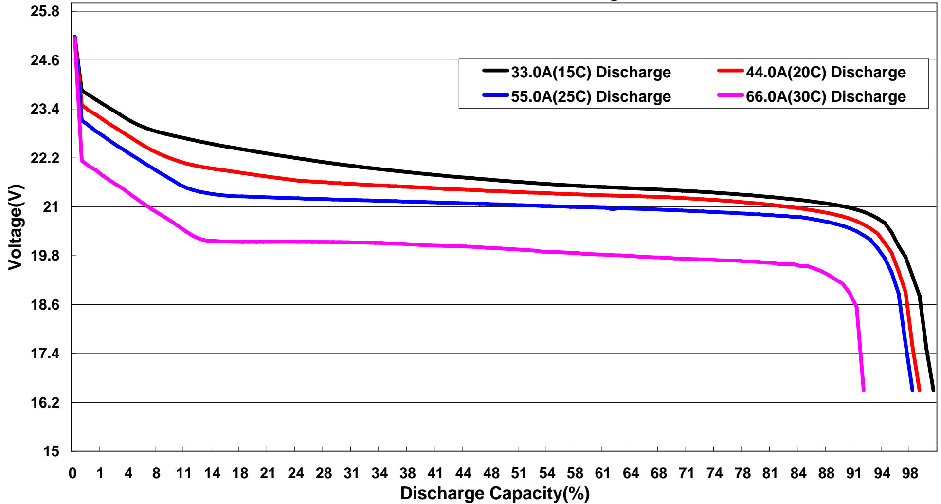
FB2200XP-6S 15C-30C Discharge Curves
