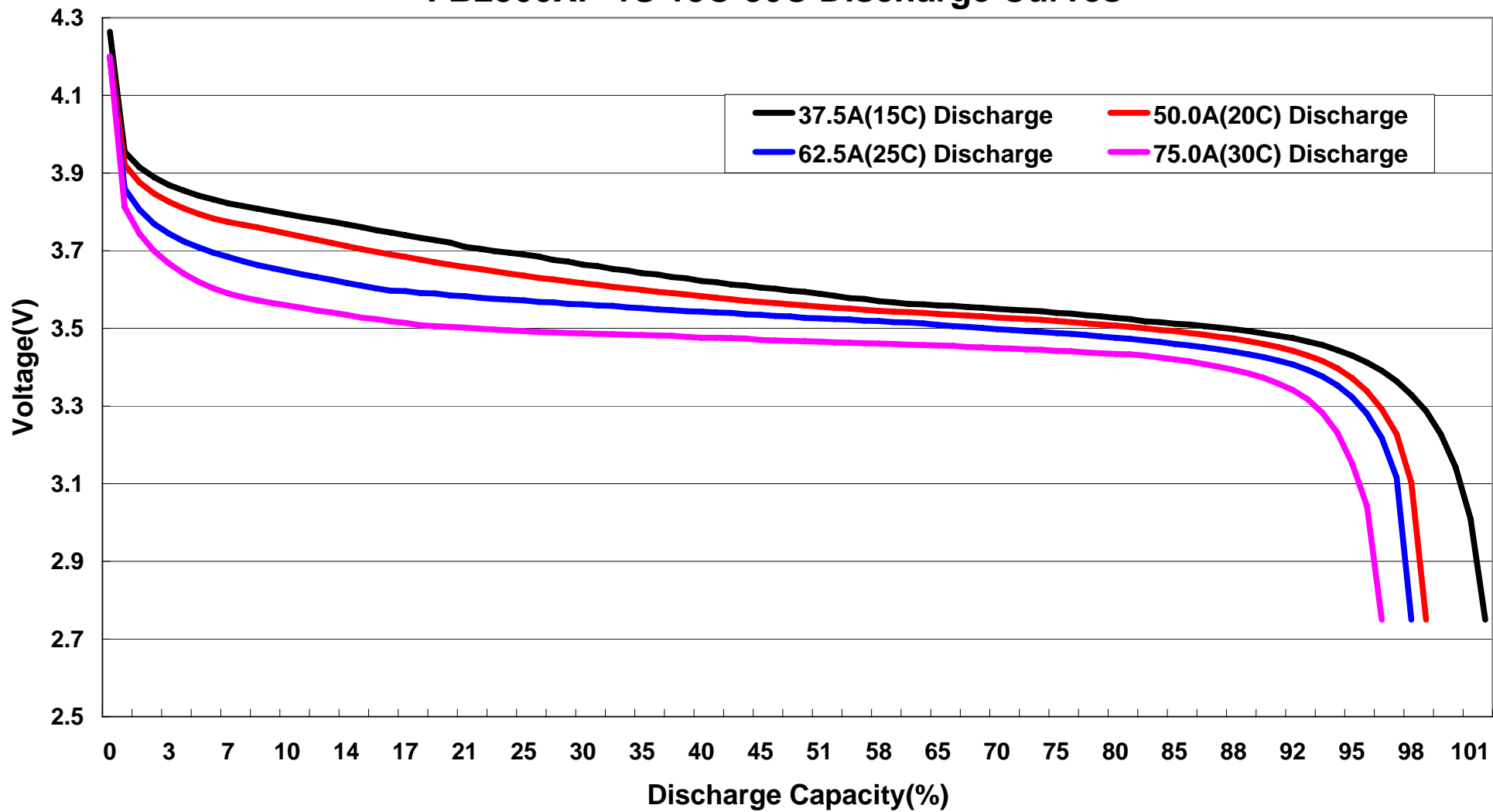
FB2500XP-1S 15C-30C Discharge Curves
