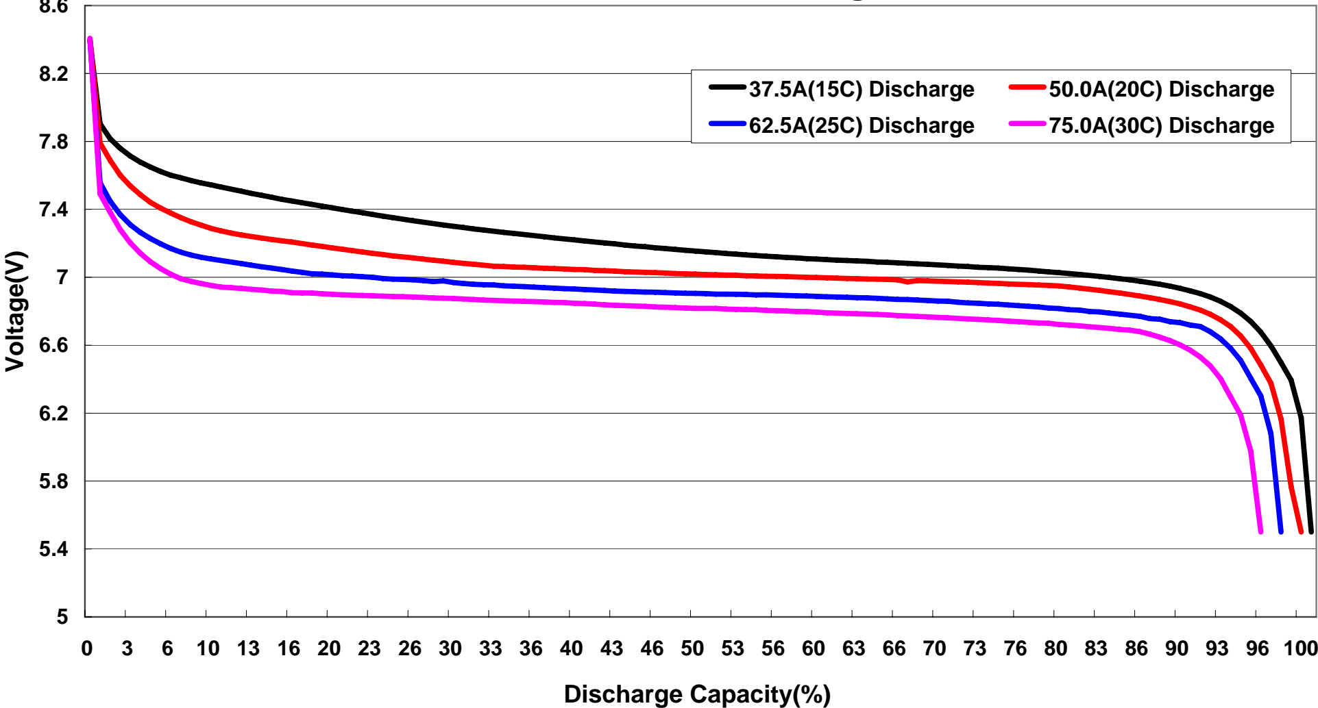
FB2500XP-2S 15C-30C Discharge Curves
