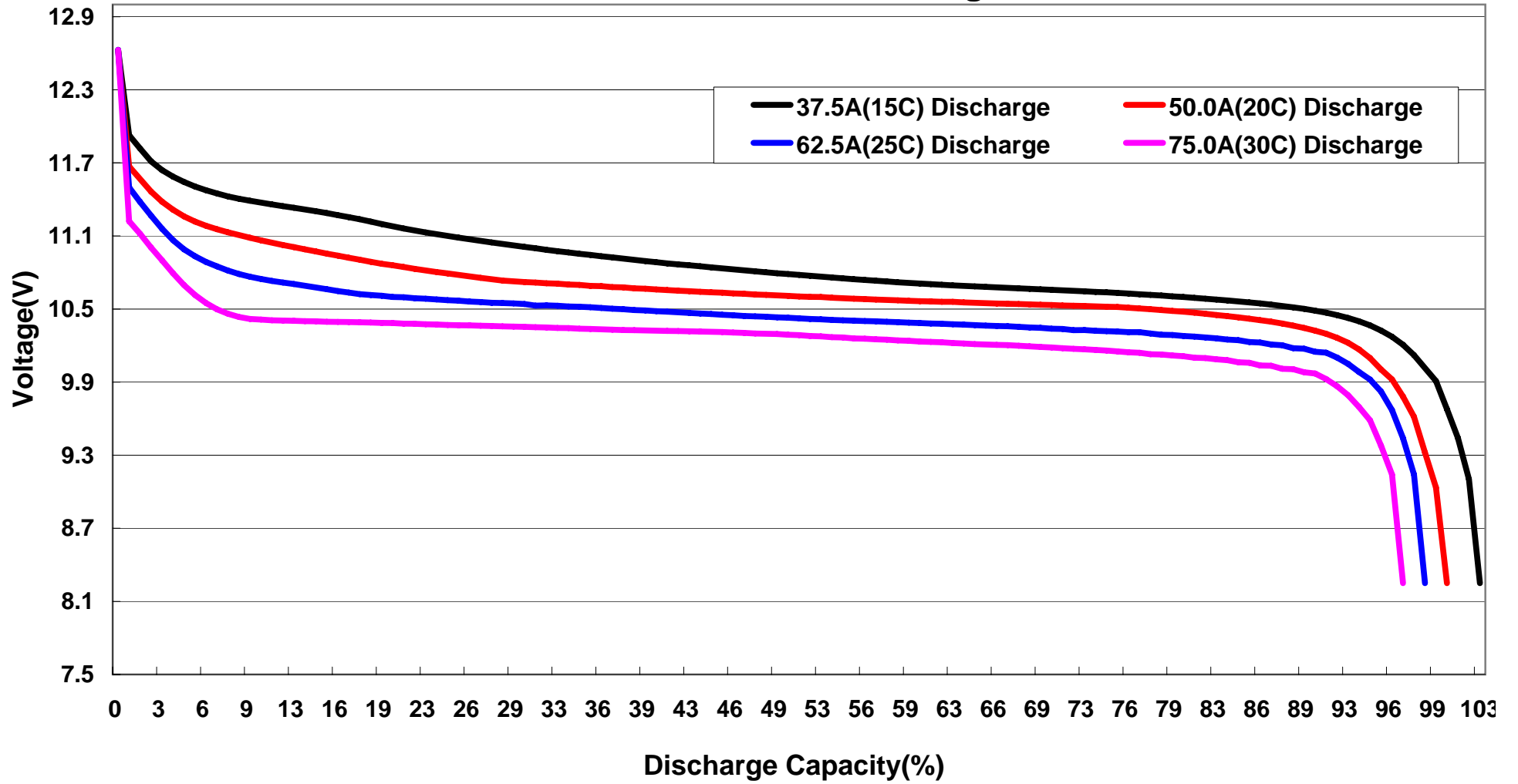
FB2500XP-3S 15C-30C Discharge Curves
