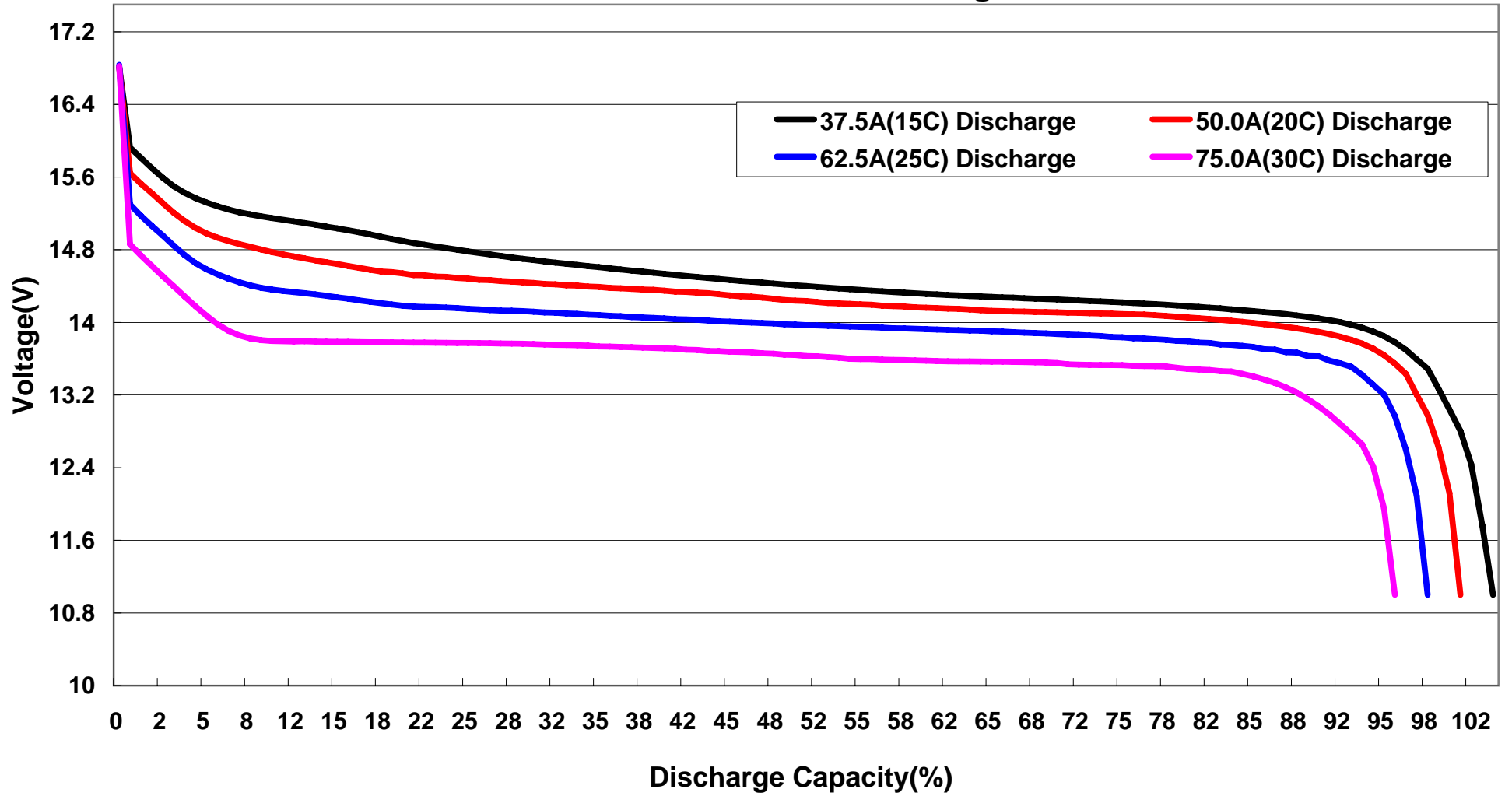
FB2500XP-4S 15C-30C Discharge Curves
