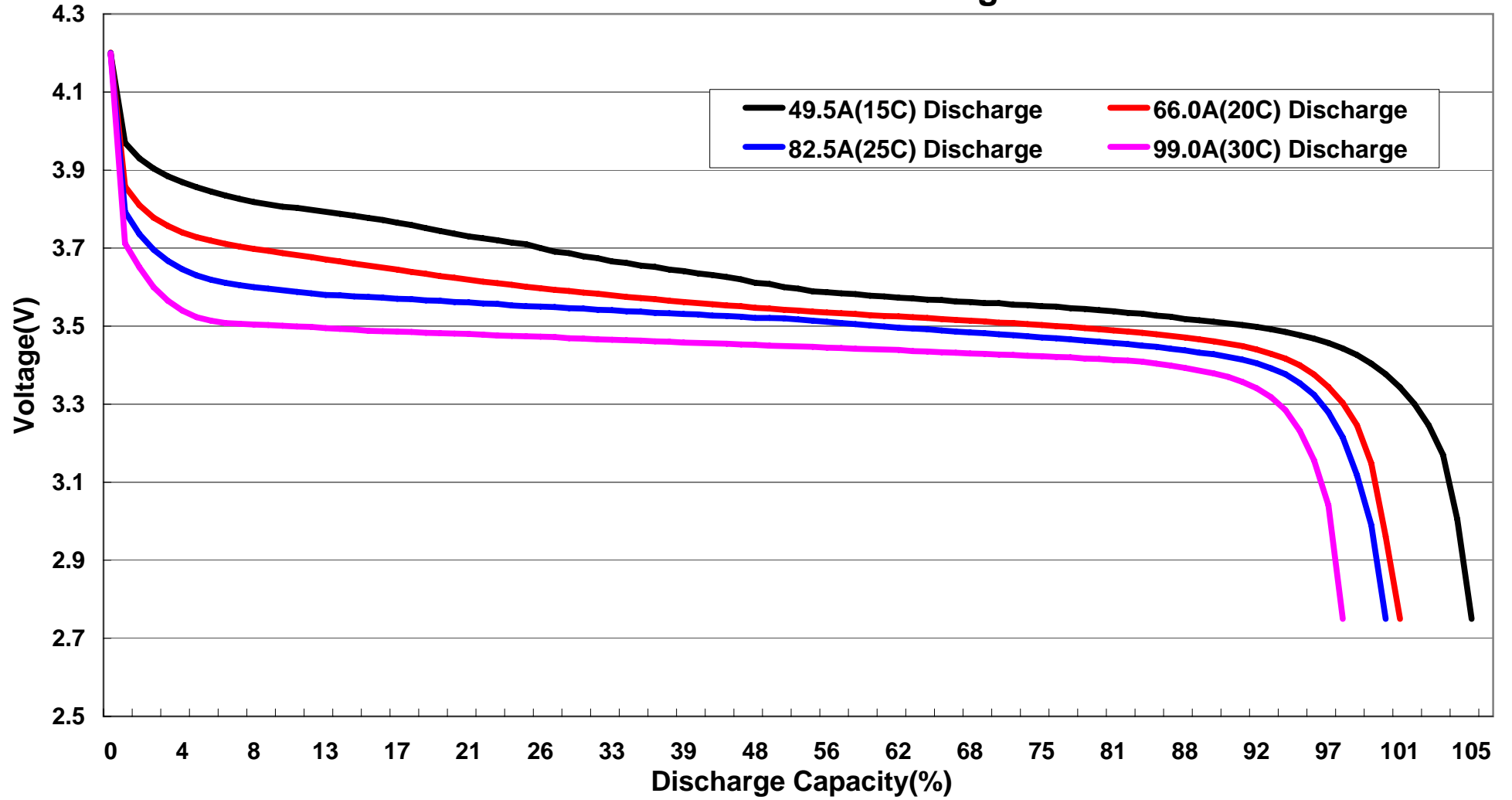
FB3300XP-1S 15C-30C Discharge Curves
