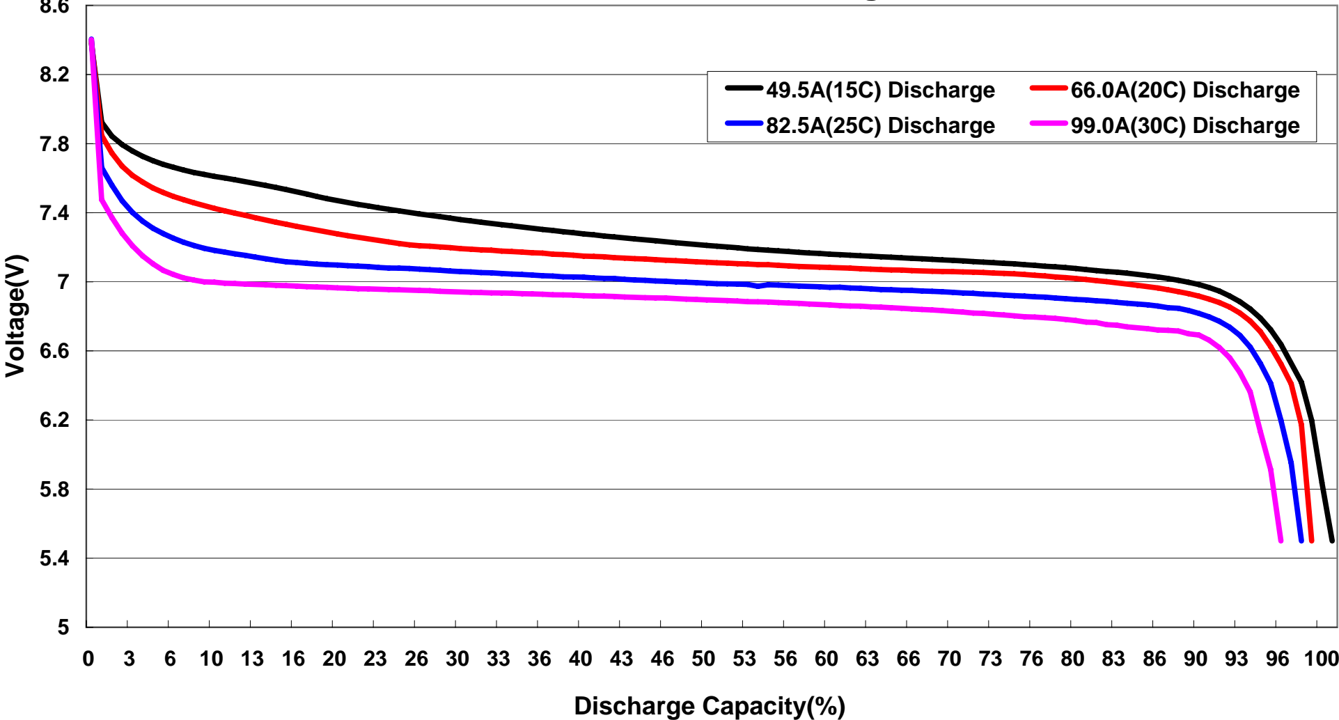
FB3300XP-2S 15C-30C Discharge Curves
