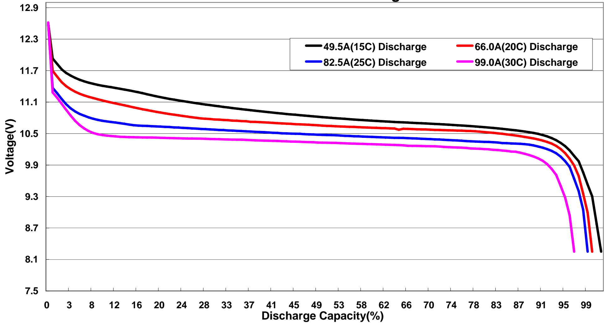
FB3300XP-3S 15C-30C Discharge Curves
