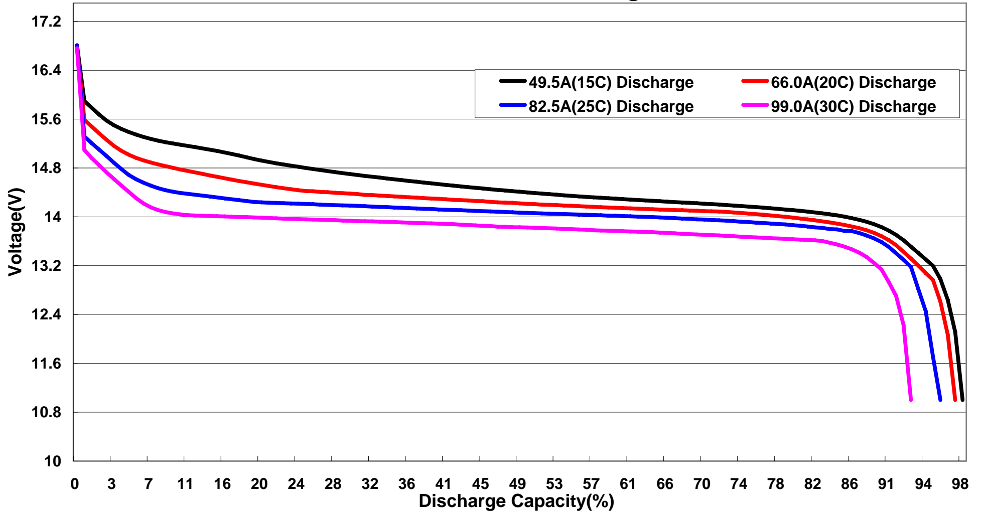
FB3300XP-4S 15C-30C Discharge Curves
