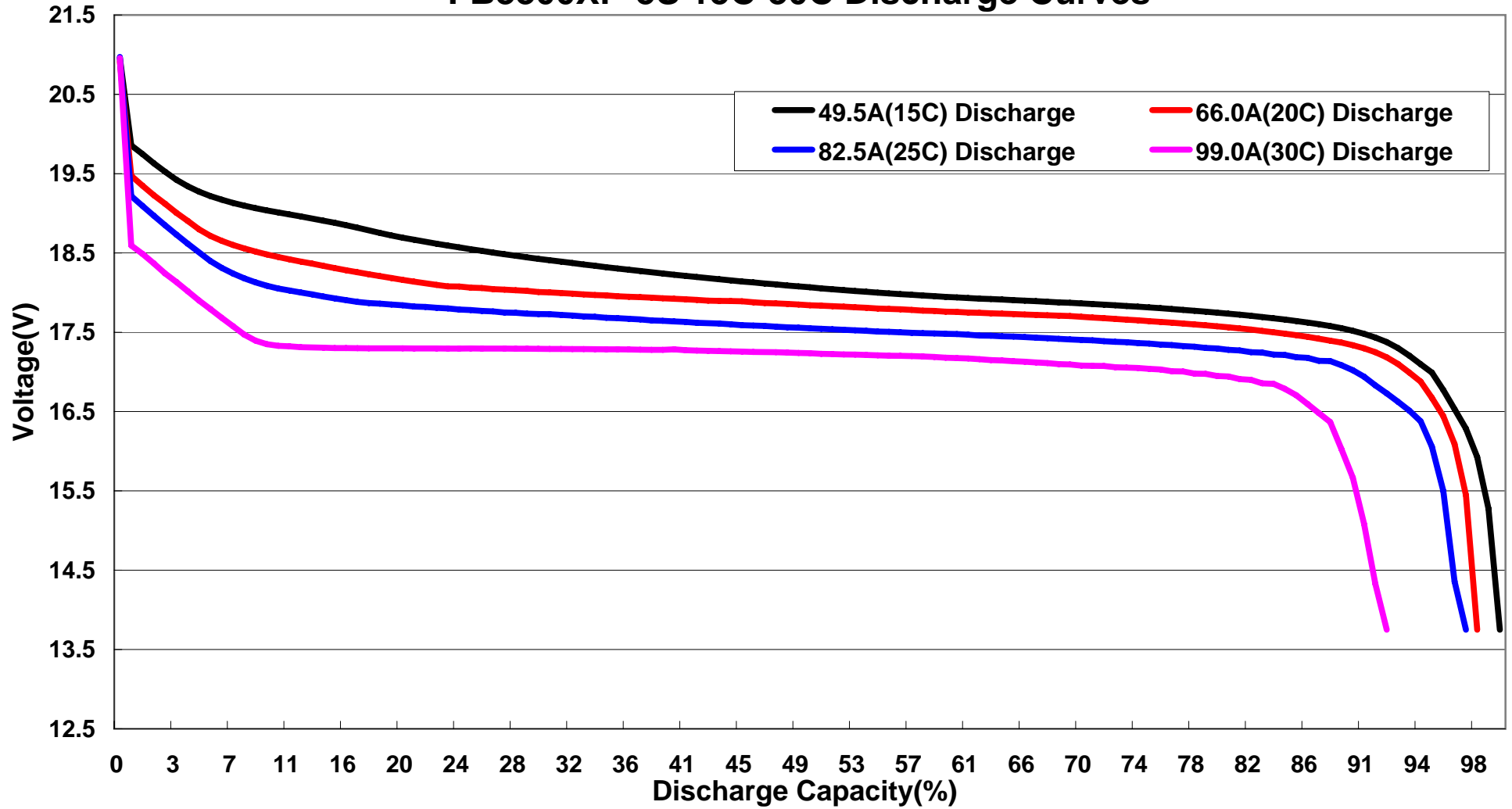
FB3300XP-5S 15C-30C Discharge Curves
