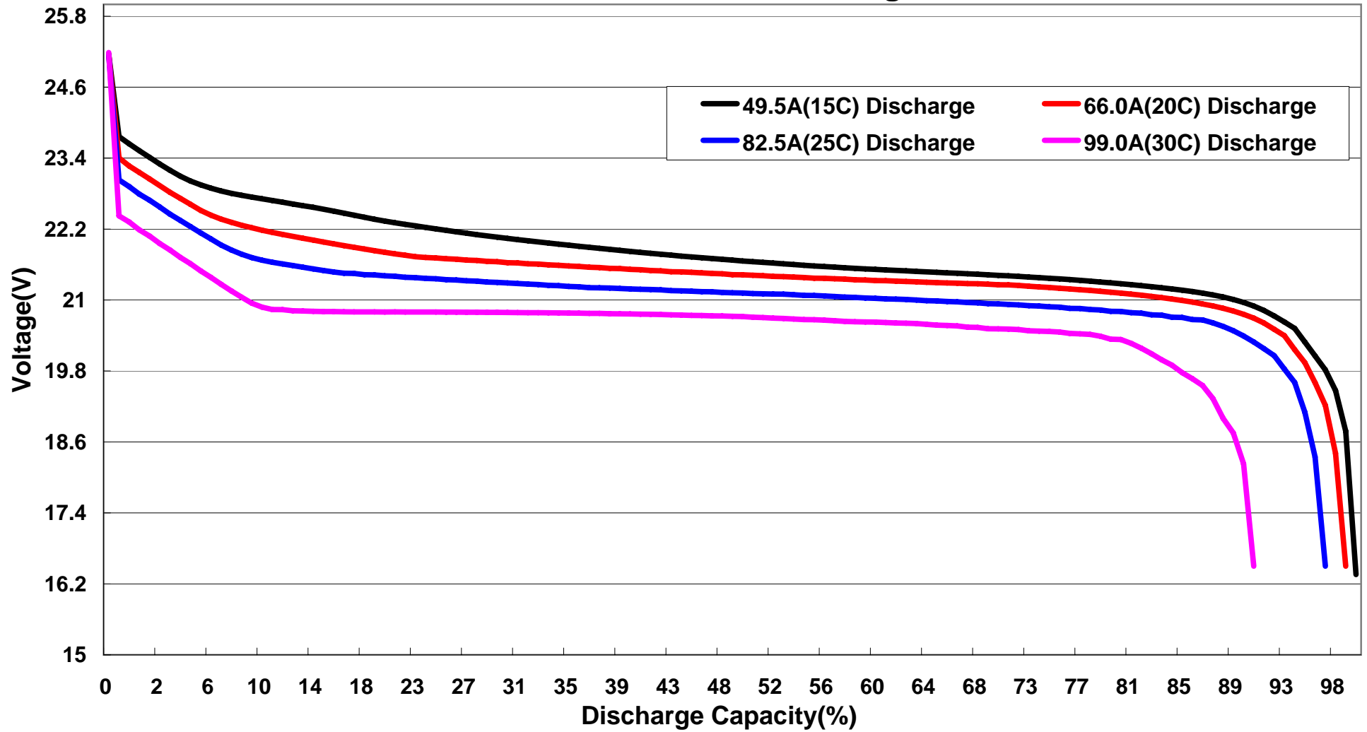
FB3300XP-6S 15C-30C Discharge Curves
