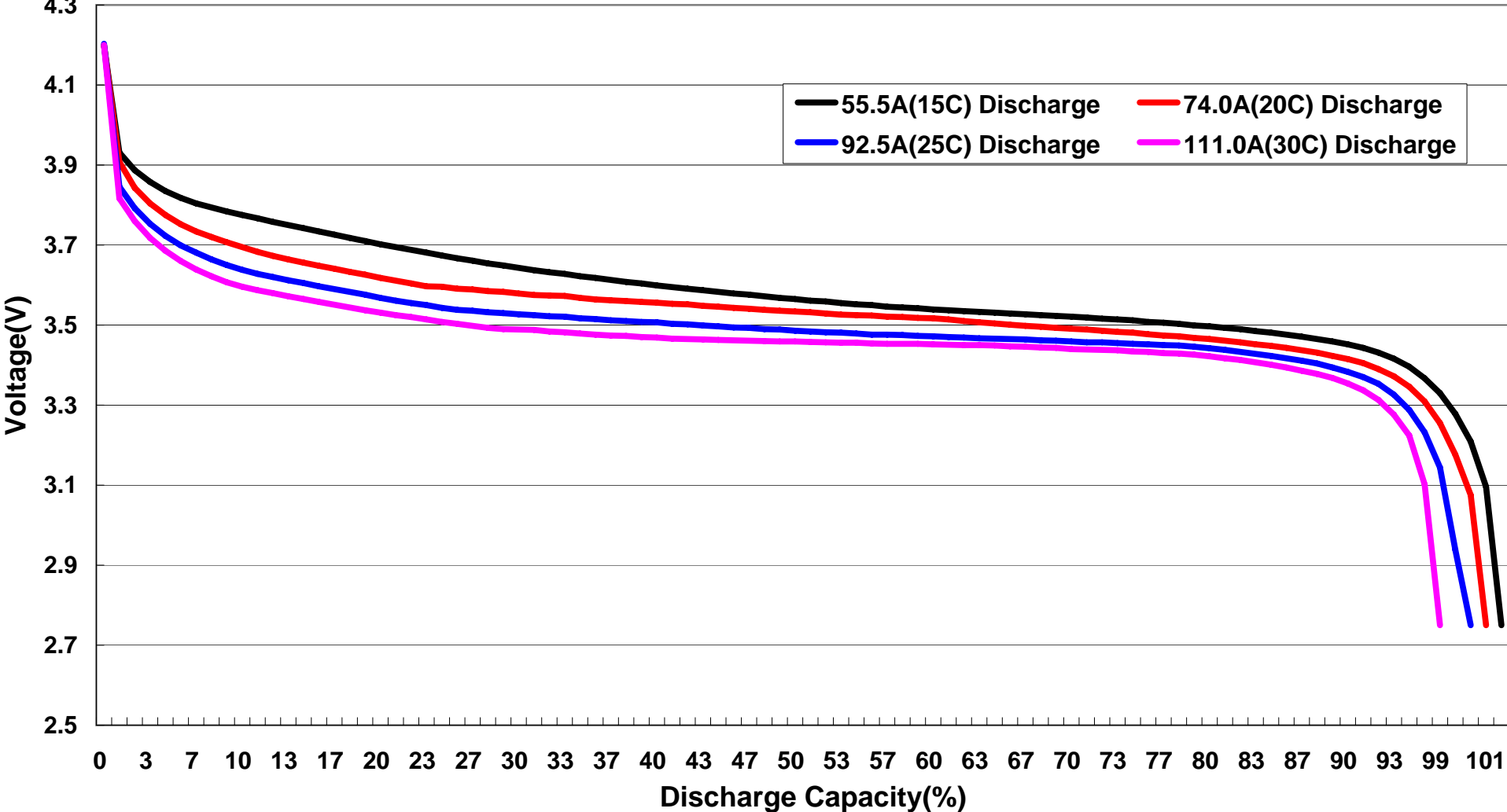
FB3700XP-1S 15C-30C Discharge Curves
