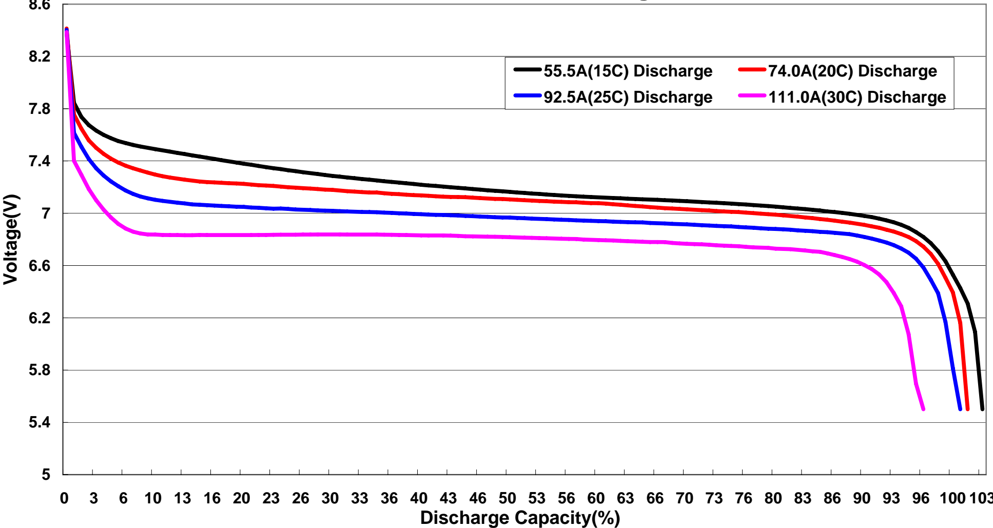
FB3700XP-2S 15C-30C Discharge Curves
