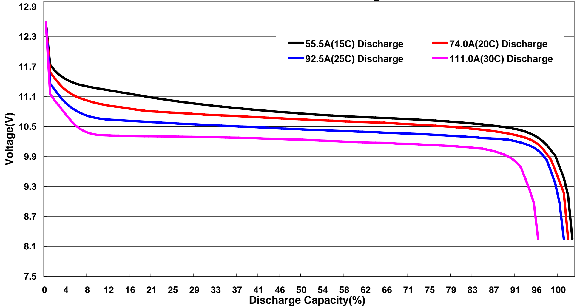
FB3700XP-3S 15C-30C Discharge Curves
