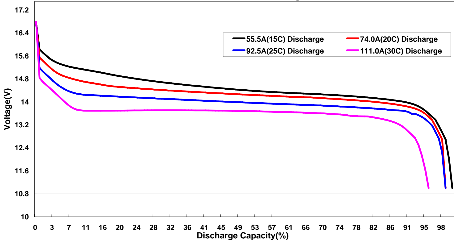
FB3700XP-4S 15C-30C Discharge Curves
