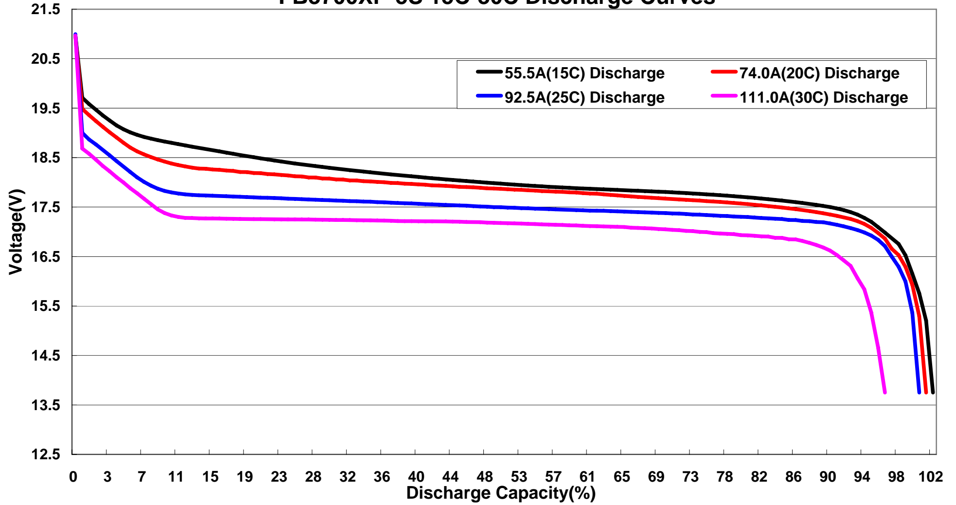
FB3700XP-5S 15C-30C Discharge Curves
