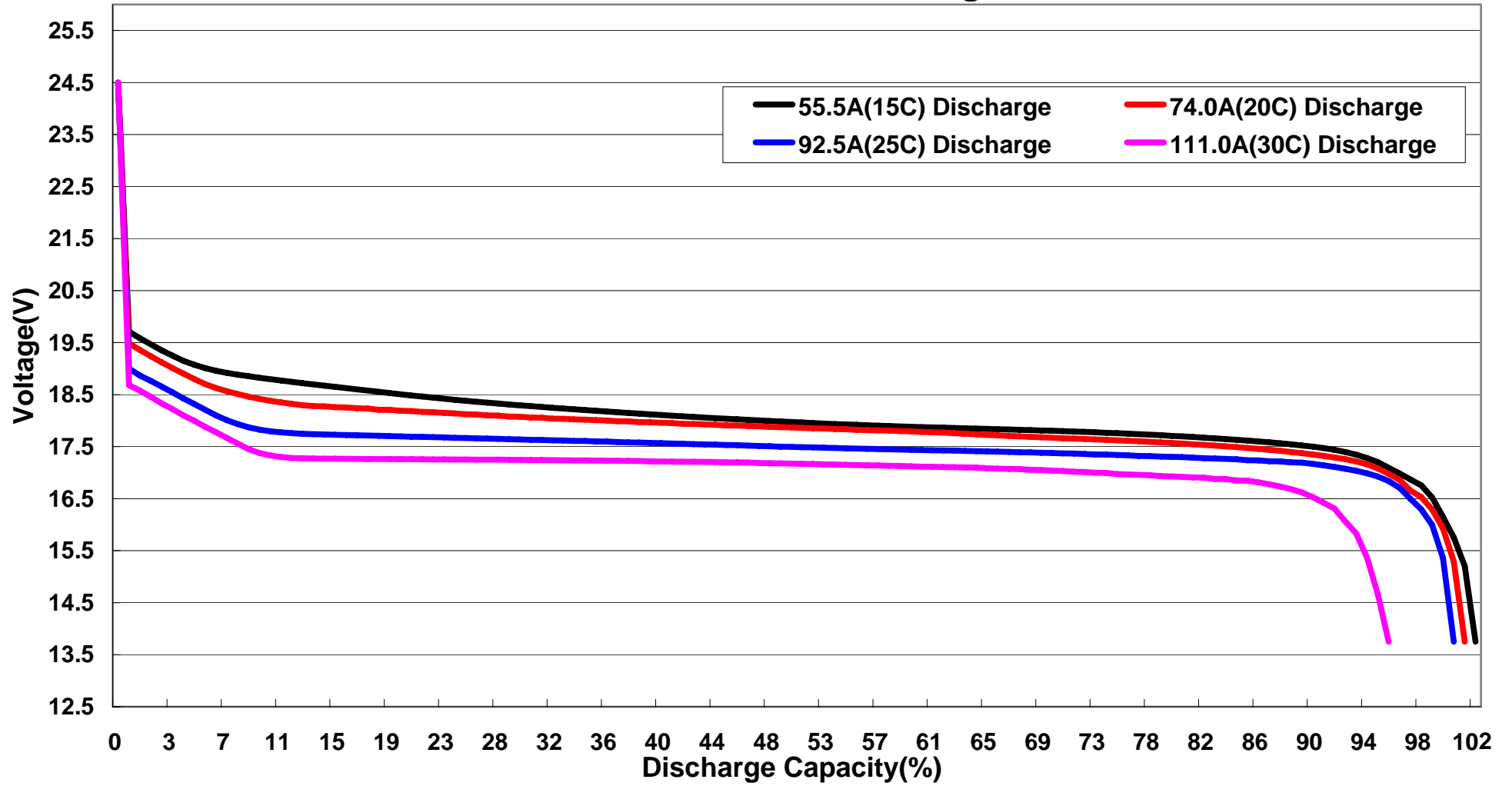
FB3700XP-6S 15C-30C Discharge Curves
