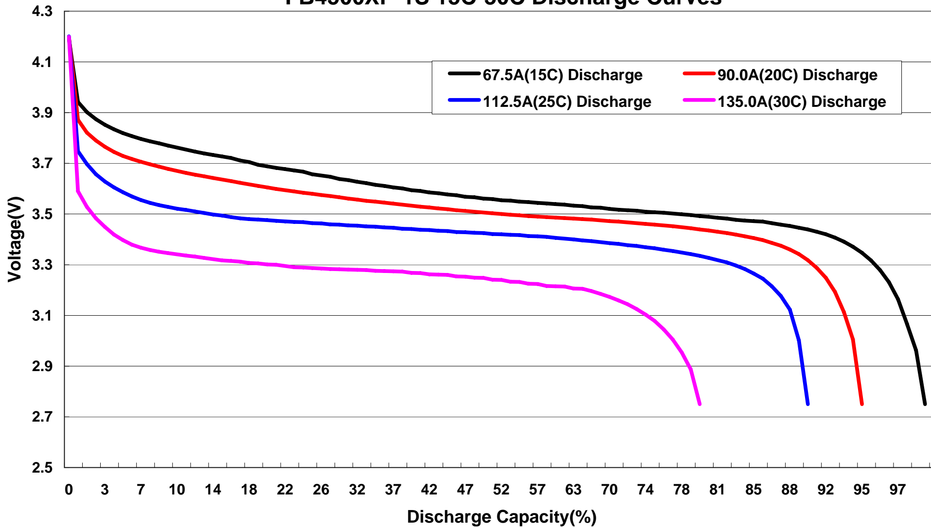
FB4500XP-1S 15C-30C Discharge Curves
