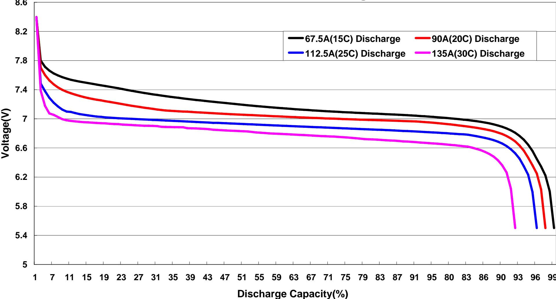
FB4500XP-2S 15C-30C Discharge Curves
