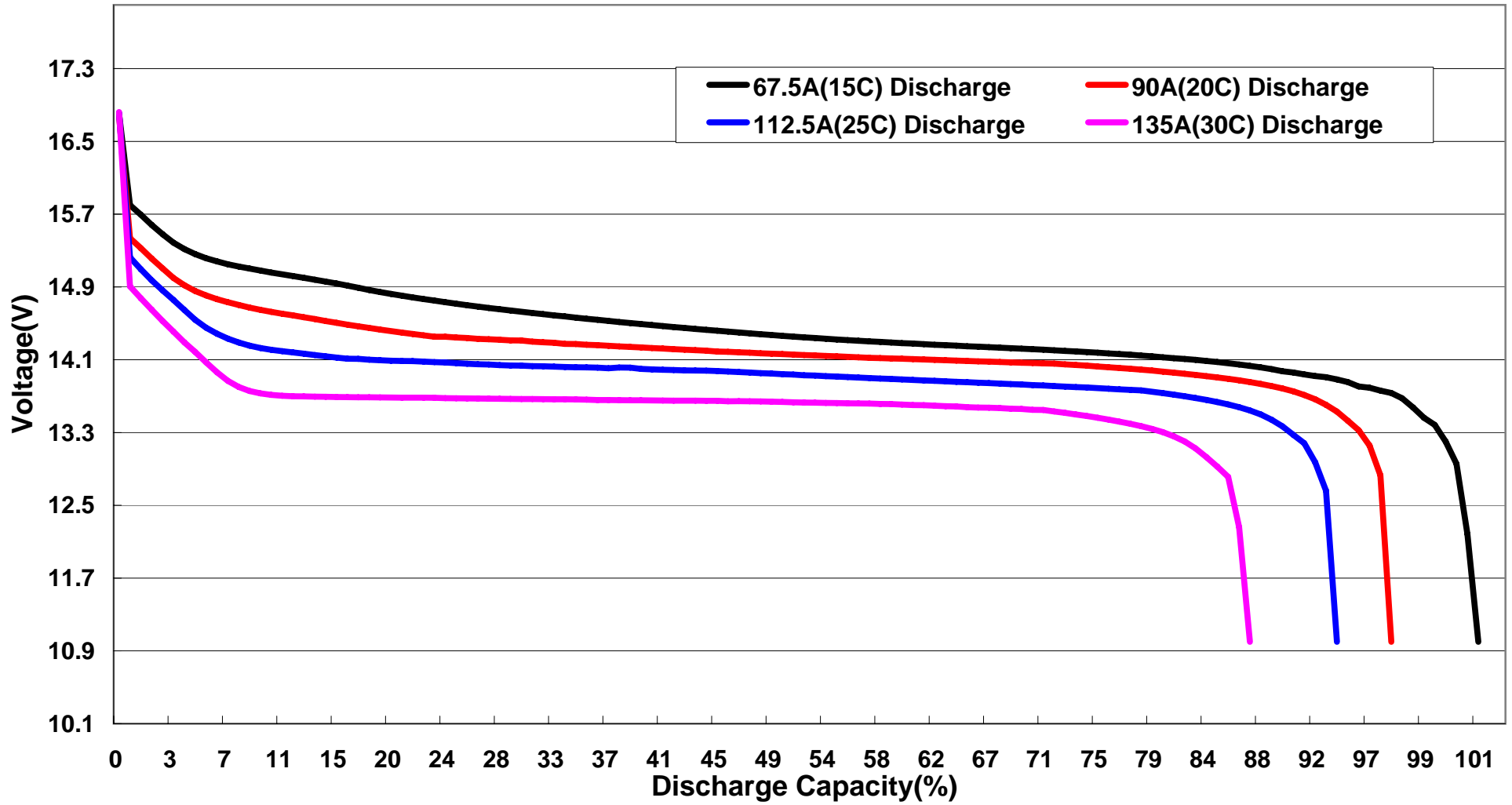
FB4500XP-4S 15C-30C Discharge Curves
