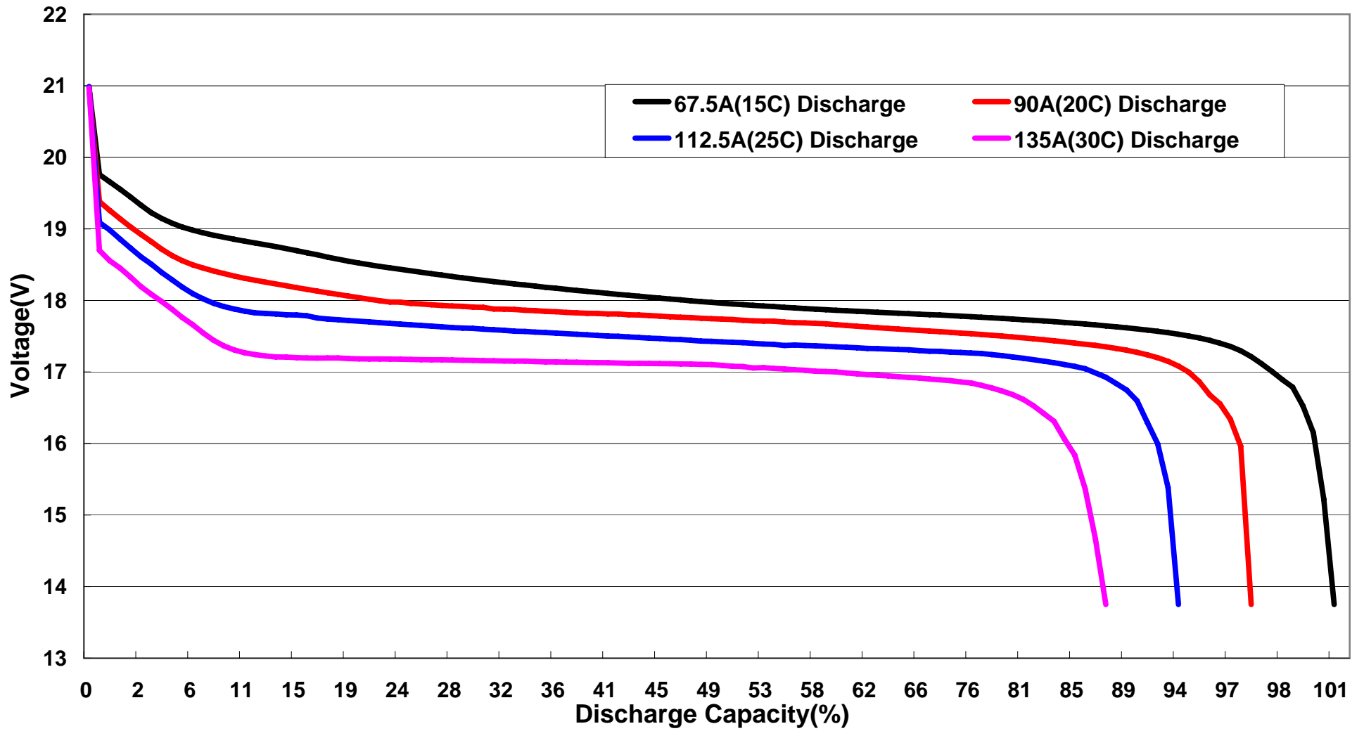
FB4500XP-5S 15C-30C Discharge Curves
