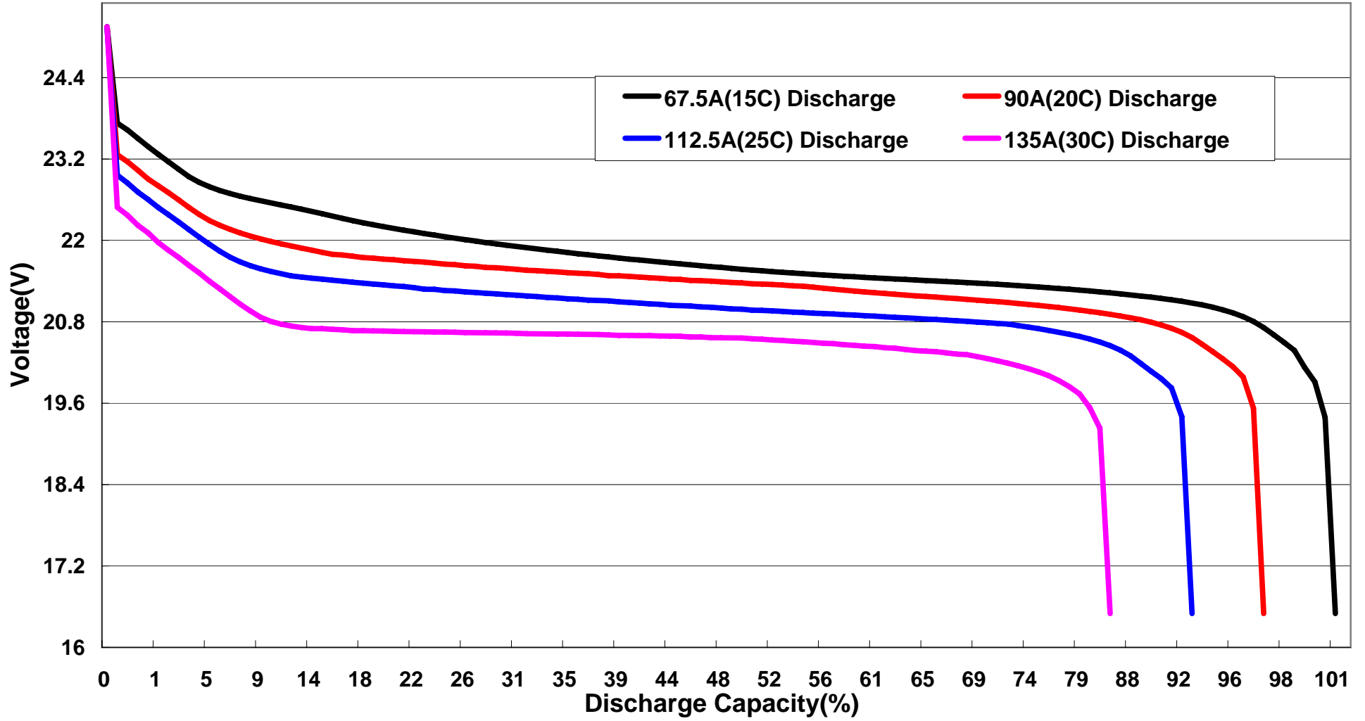
FB4500XP-6S 15C-30C Discharge Curves
