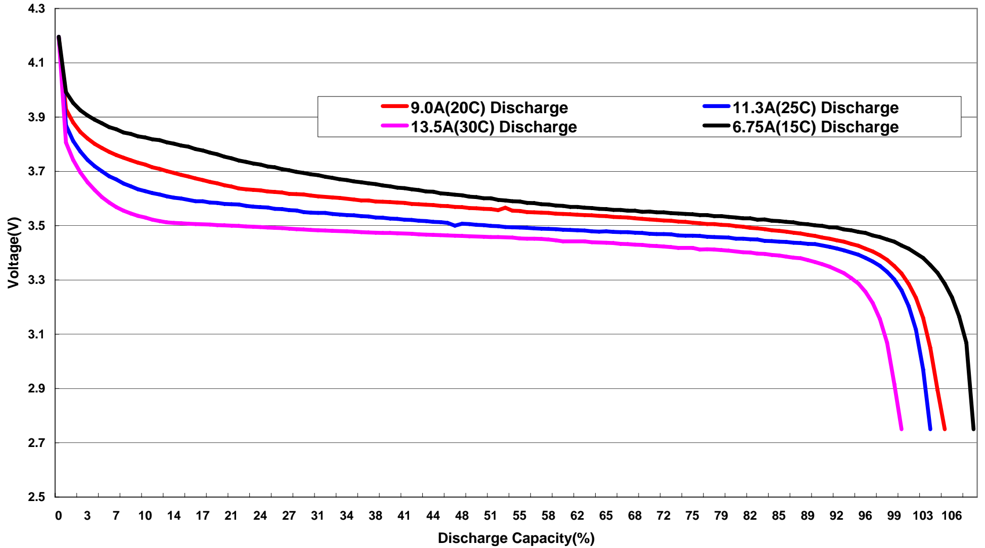
FB450XP-1S 20C-30C Discharge Curves
