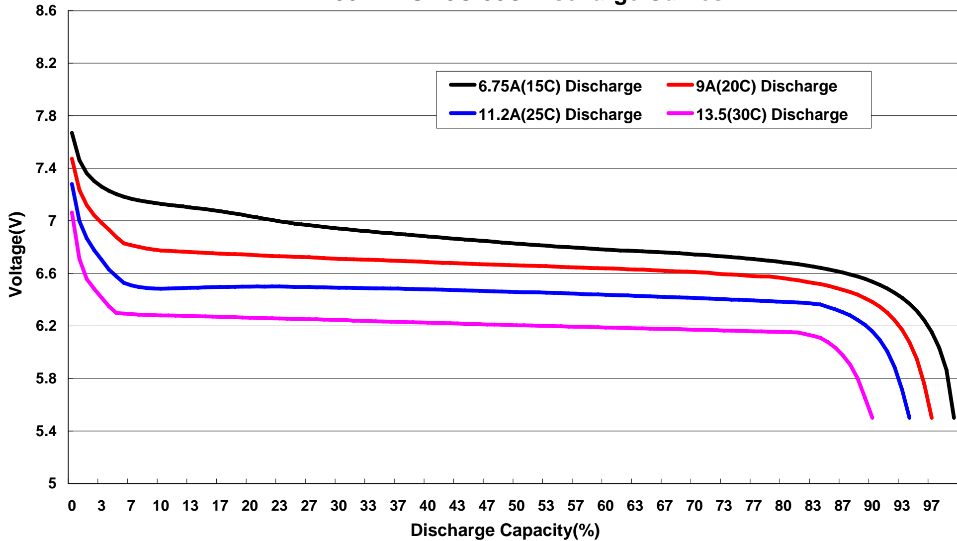
FB450XP-2S 15C-30C Discharge Curves
