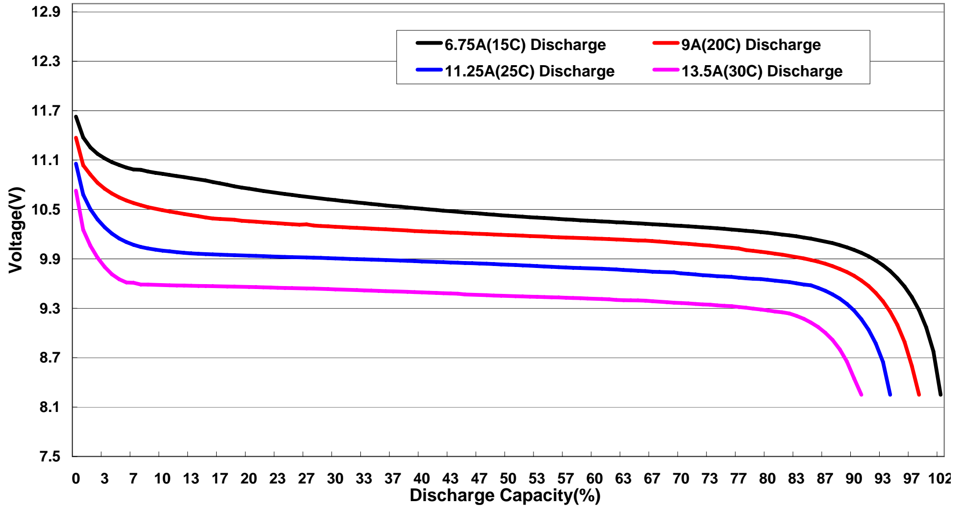
FB450XP-3S 15C-30C Discharge Curves
