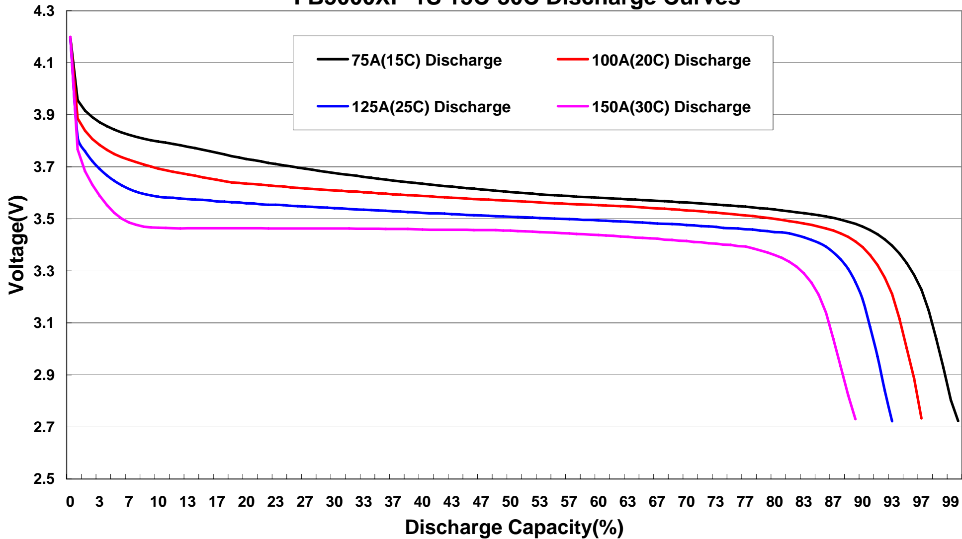
FB5000XP-1S 15C-30C Discharge Curves
