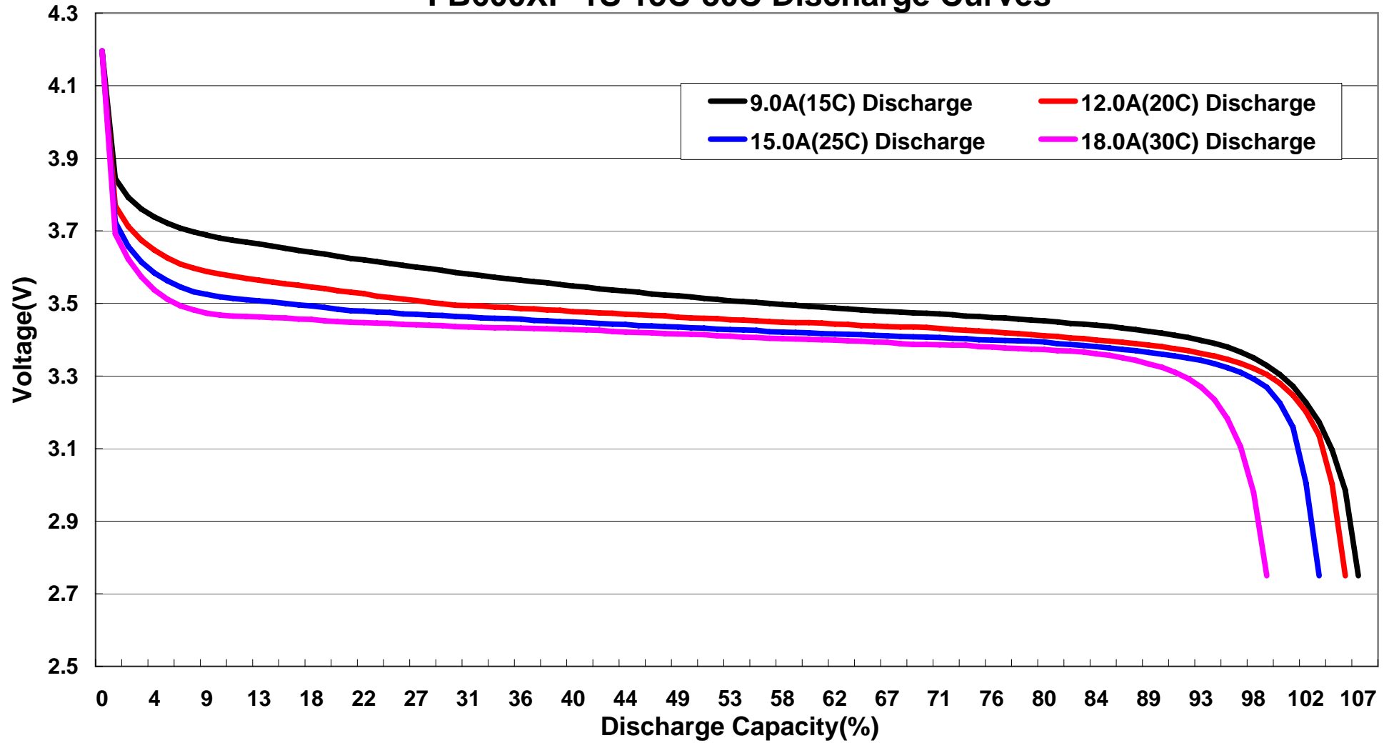
FB600XP-1S 15C-30C Discharge Curves
