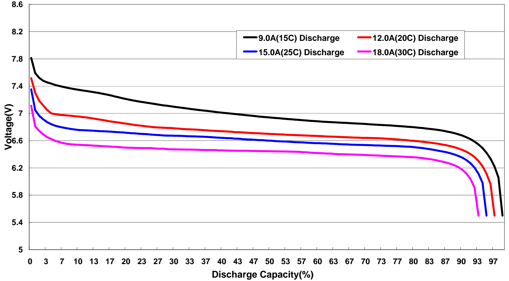
FB600XP-2S 15C-30C Discharge Curves
