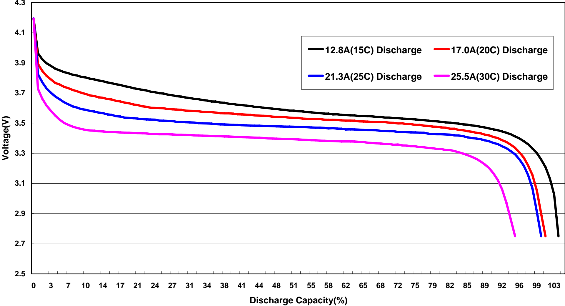
FB850XP-1S 15C-30C Discharge Curves
